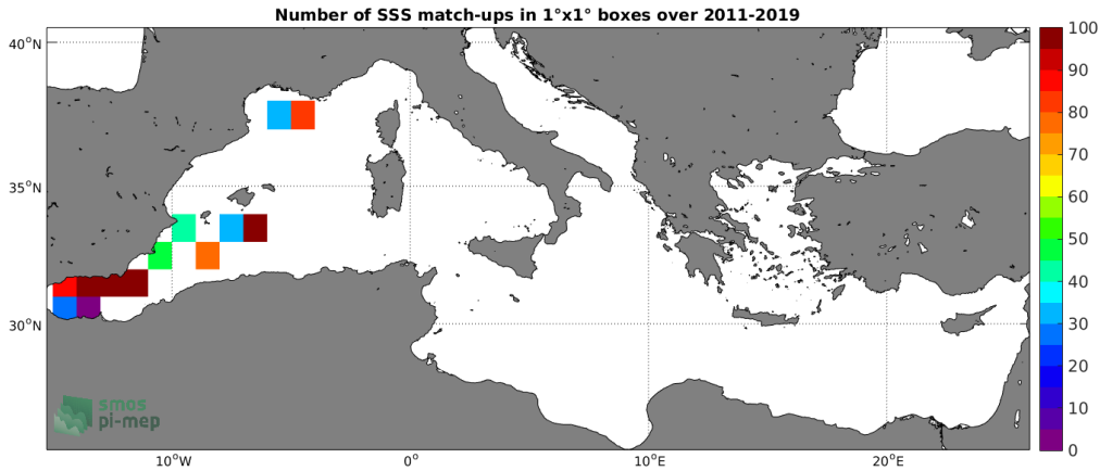
Figure 4: Number of SSS match-ups between TSG (GOSUD-Research-vessel) SSS and the SMOS SSS L2 v700 (ESA) SSS product for the Mediterranean Sea Pi-MEP region over 1^{\circ} \times 1^{\circ} boxes and for the full satellite product period.
