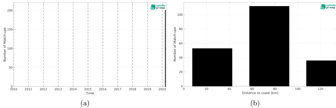
Figure 2: Number of match-ups between Saildrone and SMOS SSS L2 v700 (ESA) SSS as a function of time (a) and as function of the distance to coast (b) over the Mediterranean Sea Pi-MEP region and for the full satellite product period.
