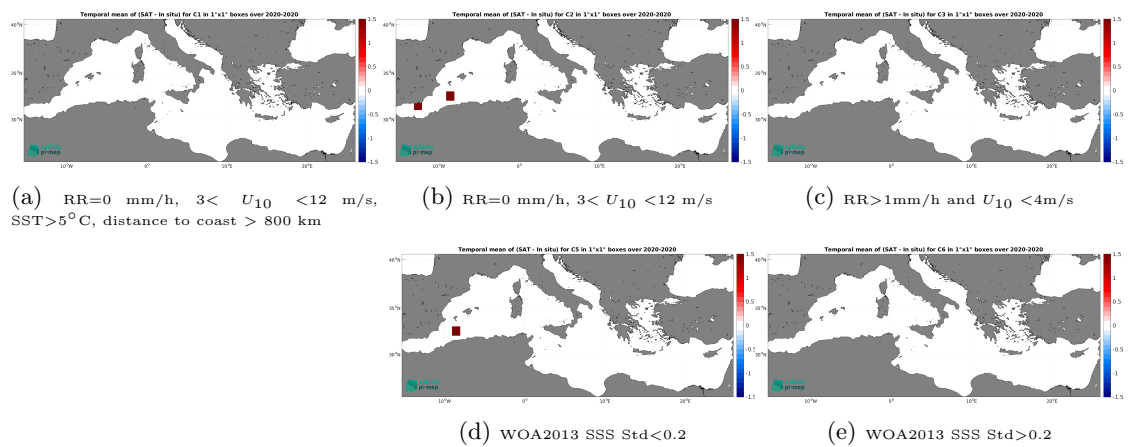
Figure 14: Temporal mean gridded over spatial boxes of size 1^\circ \times 1^\circ of \Delta\text{SSS} (SMOS SSS L2 v700 (ESA) - Saldrone) for 5 different subdatasets corresponding to:RR=0 mm/h, 3 < U_{10} < 12 m/s, SST >5^\circ\text{C} , distance to coast > 800 km (a), RR=0 mm/h, 3 < U_{10} < 12 m/s (b), RR >1 mm/h and U_{10} < 4 m/s (c), WOA2013 SSS Std <0.2 (d), WOA2013 SSS Std >0.2 (e).
