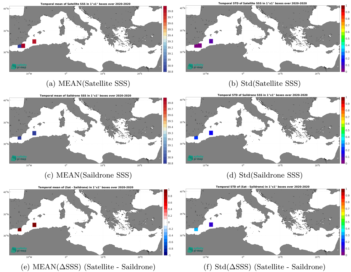
Figure 7: Temporal mean (left) and Std (right) of SSS from SMOS SSS L2 v700 (ESA) (top), Saildrone (middle), and of \Delta SSS (Satellite - Saildrone). Only match-up pairs are used to generate these maps.
