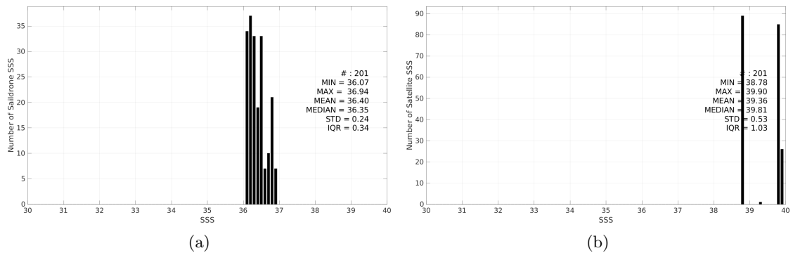
Figure 3: Histograms of SSS from Saildrone (a) and SMOS SSS L2 v700 (ESA) (b) considering all match-up pairs per bins of 0.1 over the Mediterranean Sea Pi-MEP region and for the full satellite product period.
