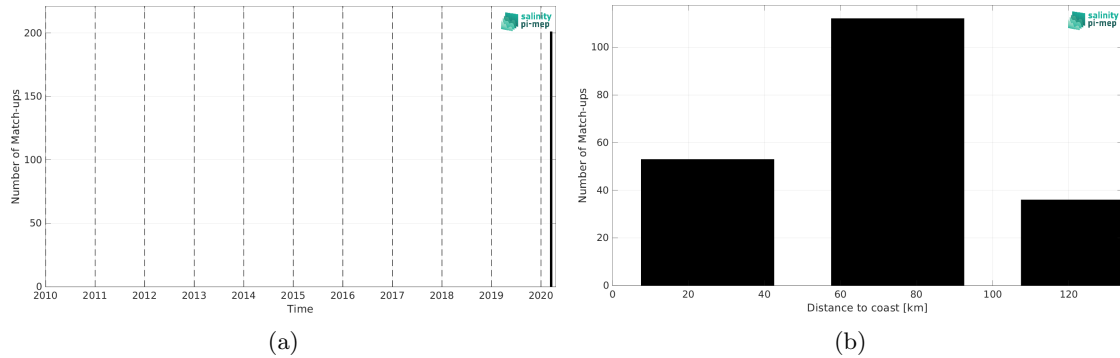
Figure 1: Number of match-ups between Saildrone and SMOS SSS L2 v700 (ESA) SSS as a function of time (a) and as function of the distance to coast (b) over the Mediterranean Sea Pi-MEP region and for the full satellite product period.
