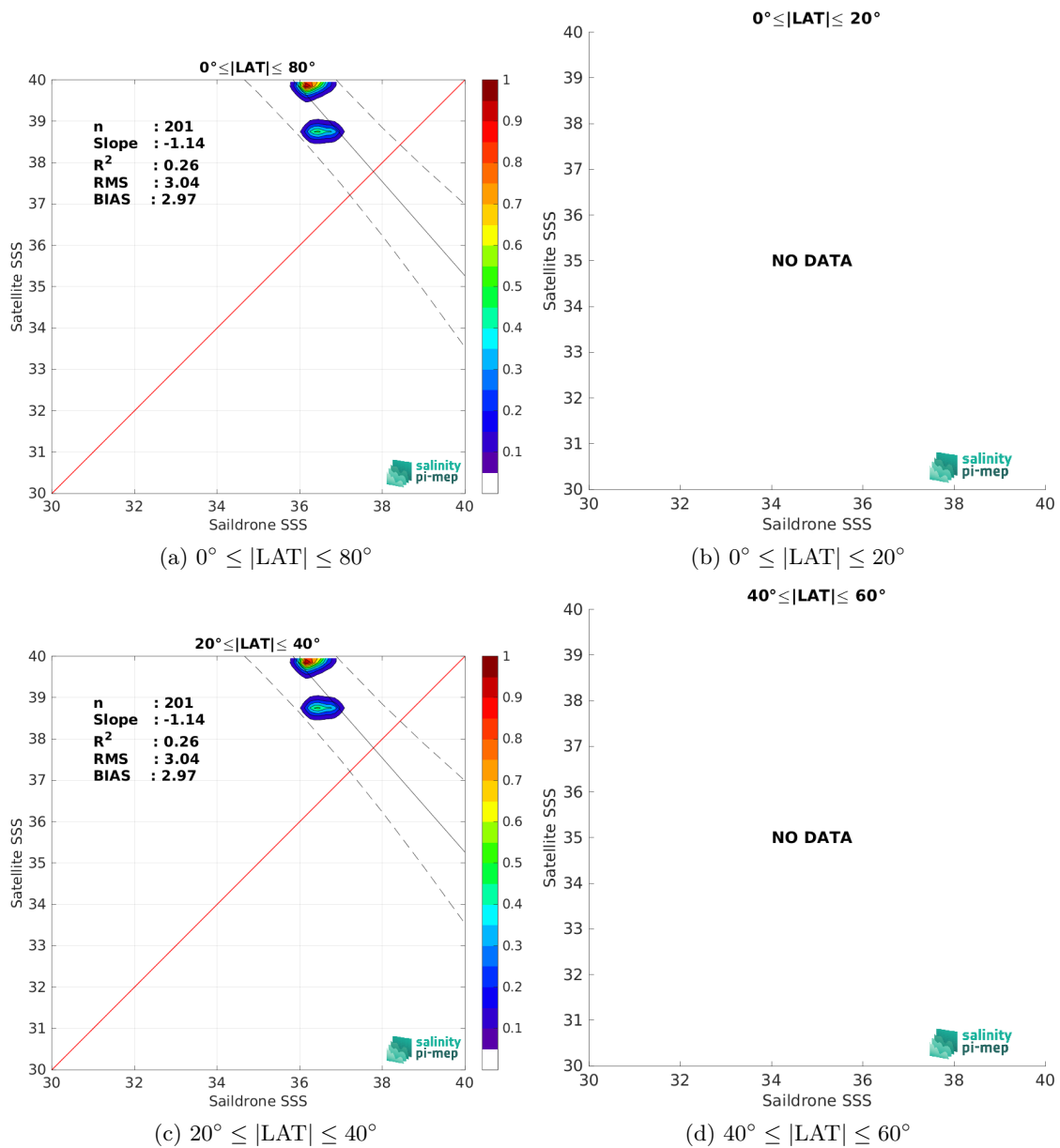
Figure 9: Contour maps of the concentration of SMOS SSS L2 v700 (ESA) SSS (y-axis) versus Saildrone SSS (x-axis) at match-up pairs for different latitude bands. For each plot, the red line shows x=y . The black thin and dashed lines indicate a linear fit through the data cloud and the \pm 95\% confidence levels, respectively. The number match-up pairs n , the slope and R^2 coefficient of the linear fit, the root mean square (RMS) and the mean bias between satellite and in situ data are indicated for each latitude band in each plots.
