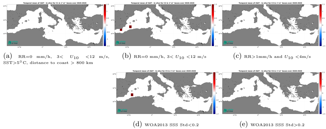
Figure 12: Temporal mean gridded over spatial boxes of size 1^{\circ}\times 1^{\circ} of \Delta\text{SSS} (SMOS SSS L2 v700 (ESA) - Saildrone) for 5 different subdatasets corresponding to:RR=0 mm/h, 3 < U_{10} < 12 m/s, SST > 5^{\circ}\text{C} , distance to coast > 800 km (a), RR=0 mm/h, 3 < U_{10} < 12 m/s (b), RR > 1 mm/h and U_{10} < 4 m/s (c), WOA2013 SSS Std < 0.2 (d), WOA2013 SSS Std > 0.2 (e).
