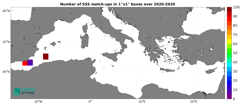
Figure 4: Number of SSS match-ups between Saildrone SSS and the SMOS SSS L2 v700 (ESA) SSS product for the Mediterranean Sea Pi-MEP region over 1^\circ \times 1^\circ boxes and for the full satellite product period.
