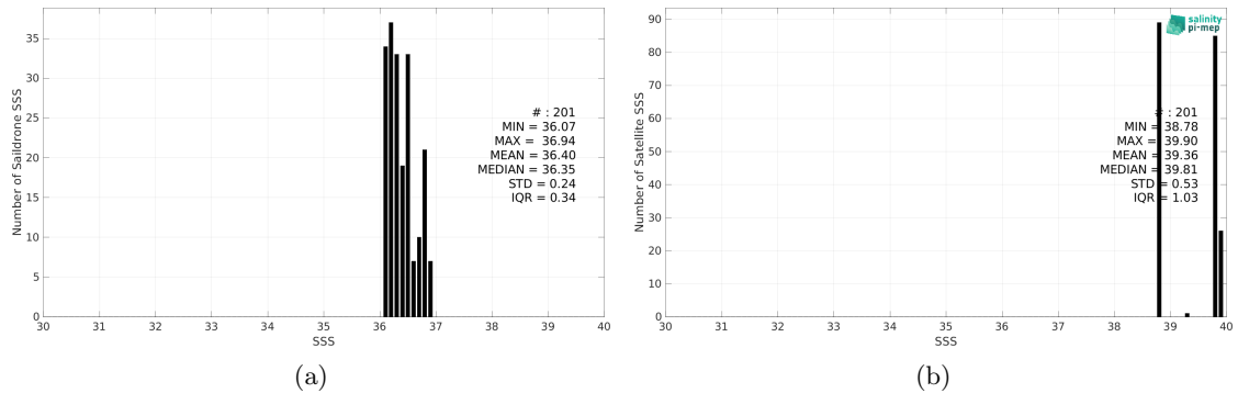
Figure 2: Histograms of SSS from Saildrone (a) and SMOS SSS L2 v700 (ESA) (b) considering all match-up pairs per bins of 0.1 over the Mediterranean Sea Pi-MEP region and for the full satellite product period.
