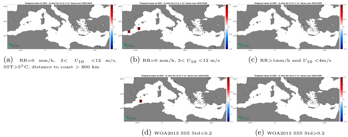
Figure 12: Temporal mean gridded over spatial boxes of size 1^{\circ}\times 1^{\circ} of \Delta\text{SSS} (SMOS SSS L2 v700 (ESA) - Sairdrone) for 5 different subdatasets corresponding to: RR=0 mm/h, 3 < U_{10} < 12 m/s, SST > 5^{\circ}\text{C} , distance to coast > 800 km (a), RR=0 mm/h, 3 < U_{10} < 12 m/s (b), RR > 1 mm/h and U_{10} < 4 m/s (c), WOA2013 SSS Std < 0.2 (d), WOA2013 SSS Std > 0.2 (e).
