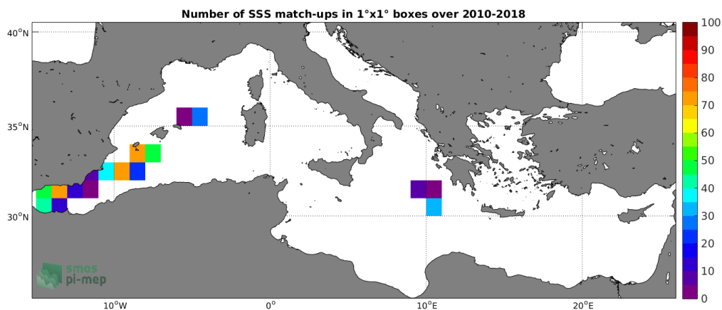
Figure 4: Number of SSS match-ups between TSG (LEGOS-DM) SSS and the SMOS SSS L2 v662 (ESA) SSS product for the Mediterranean Sea Pi-MEP region over 1^\circ \times 1^\circ boxes and for the full satellite product period.
