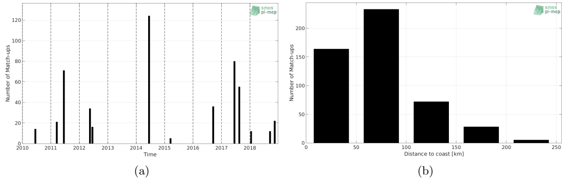
Figure 1: Number of match-ups between TSG (LEGOS-DM) and SMOS SSS L2 v662 (ESA) SSS as a function of time (a) and as function of the distance to coast (b) over the Mediterranean Sea Pi-MEP region and for the full satellite product period.
