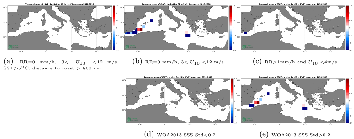
Figure 12: Temporal mean gridded over spatial boxes of size 1^\circ \times 1^\circ of \Delta SSS (SMOS SSS L2 v662 (ESA) - TSG (LEGOS-DM)) for 5 different subdatasets corresponding to: RR=0 mm/h, 3 < U_{10} < 12 m/s, SST > 5°C, distance to coast > 800 km (a), RR=0 mm/h, 3 < U_{10} < 12 m/s (b), RR > 1mm/h and U_{10} < 4 m/s (c), WOA2013 SSS Std < 0.2 (d), WOA2013 SSS Std > 0.2 (e).
