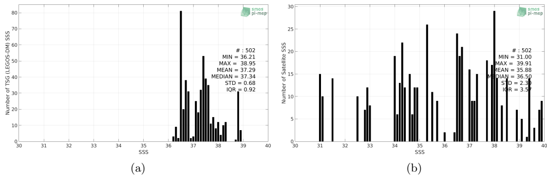
Figure 2: Histograms of SSS from TSG (LEGOS-DM) (a) and SMOS SSS L2 v662 (ESA) (b) considering all match-up pairs per bins of 0.1 over the Mediterranean Sea Pi-MEP region and for the full satellite product period.
