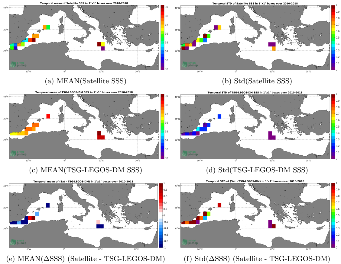
Figure 6: Temporal mean (left) and Std (right) of SSS from SMOS L2 v662 (ESA) (top), TSG-LEGOS-DM (middle), and of \Delta SSS (Satellite - TSG-LEGOS-DM). Only match-up pairs are used to generate these maps.
