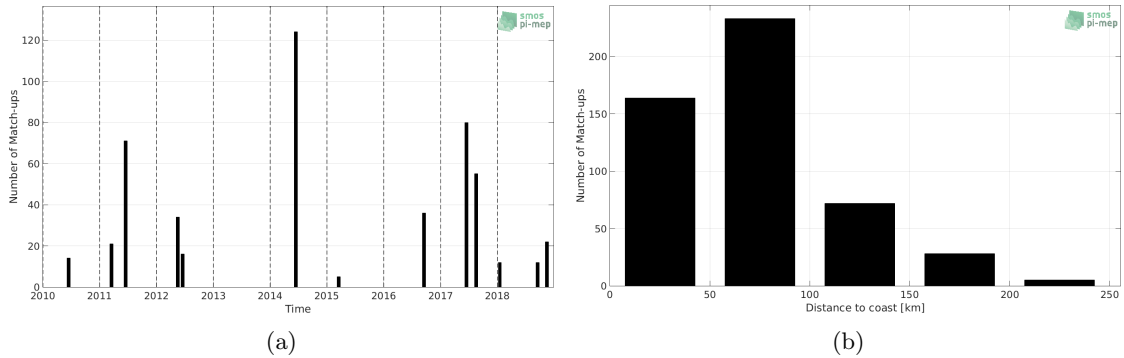
Figure 1: Number of match-ups between TSG-LEGOS-DM and SMOS L2 v662 (ESA) SSS as a function of time (a) and as function of the distance to coast (b) over the Mediterranean Sea Pi-MEP region and for the full satellite product period.
