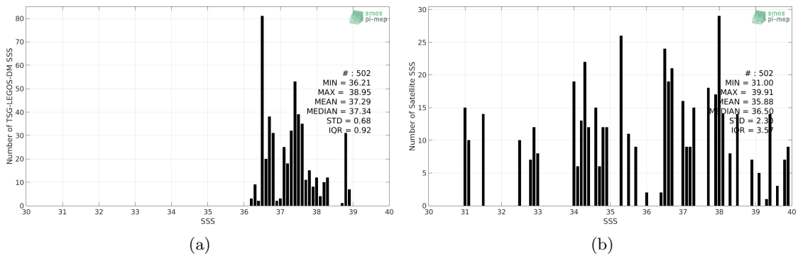
Figure 2: Histograms of SSS from TSG-LEGOS-DM (a) and SMOS L2 v662 (ESA) (b) considering all match-up pairs per bins of 0.1 over the Mediterranean Sea Pi-MEP region and for the full satellite product period.
