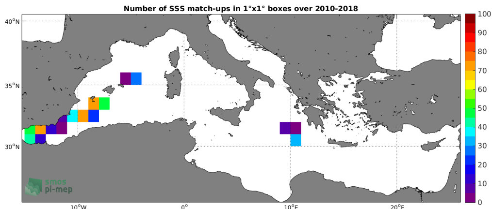
Figure 4: Number of SSS match-ups between TSG-LEGOS-DM SSS and the SMOS L2 v662 (ESA) SSS product for the Mediterranean Sea Pi-MEP region over 1^\circ \times 1^\circ boxes and for the full satellite product period.
