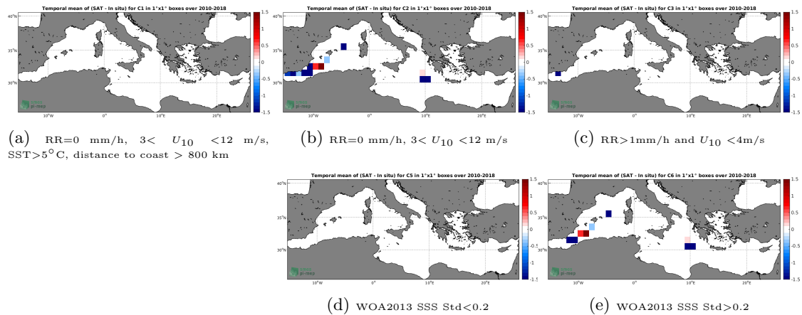
Figure 12: Temporal mean gridded over spatial boxes of size 1^\circ \times 1^\circ of \Delta SSS (SMOS-L2-DPGS-v662 - TSG-LEGOS-DM) for 5 different subdatasets corresponding to:RR=0 mm/h, 3 < U_{10} < 12 m/s, SST >5^\circ\text{C} , distance to coast > 800 km (a), RR=0 mm/h, 3 < U_{10} < 12 m/s (b), RR >1 mm/h and U_{10} < 4 m/s (c), WOA2013 SSS Std <0.2 (d), WOA2013 SSS Std >0.2 (e).
