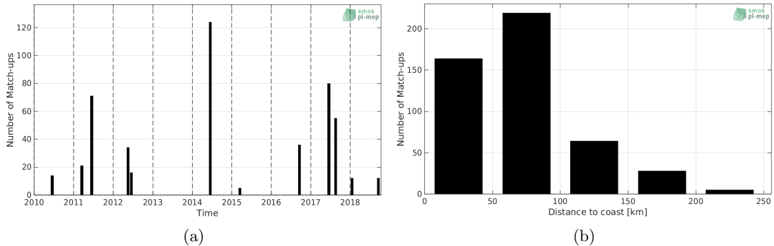
Figure 1: Number of match-ups between TSG-LEGOS-DM and SMOS-L2-DPGS-v662 SSS as a function of time (a) and as function of the distance to coast (b) over the Mediterranean Sea Pi-MEP region and for the full satellite product period.
