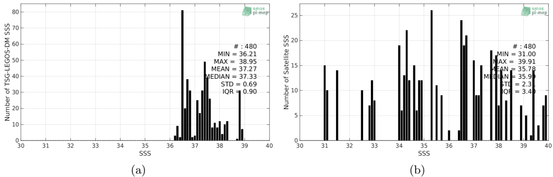
Figure 2: Histograms of SSS from TSG-LEGOS-DM (a) and SMOS-L2-DPGS-v662 (b) considering all match-up pairs per bins of 0.1 over the Mediterranean Sea Pi-MEP region and for the full satellite product period.
