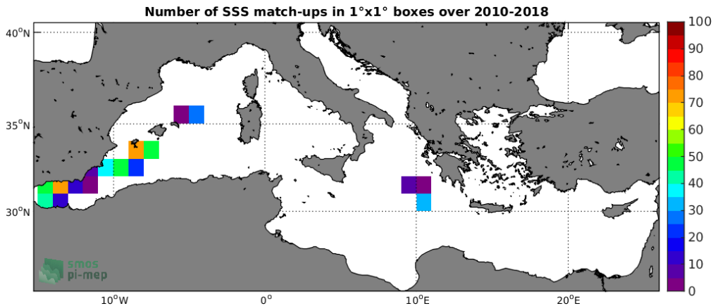
Figure 4: Number of SSS match-ups between TSG-LEGOS-DM SSS and the SMOS-L2-DPGS-v662 SSS product for the Mediterranean Sea Pi-MEP region over 1°x1° boxes and for the full satellite product period.
