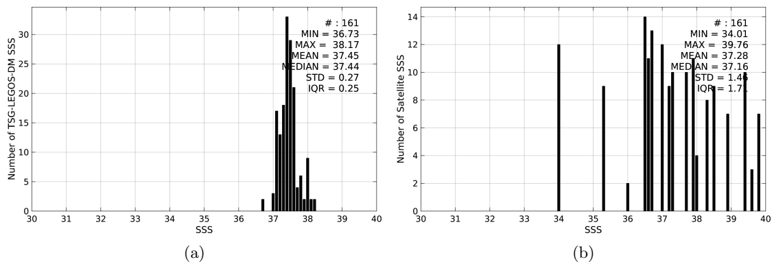
Figure 2: Histograms of SSS from TSG-LEGOS-DM (a) and SMOS-L2-DPGS-v662 (b) considering all match-up pairs per bins of 0.1 over the Mediterranean Sea Pi-MEP region and for the full satellite product period.
