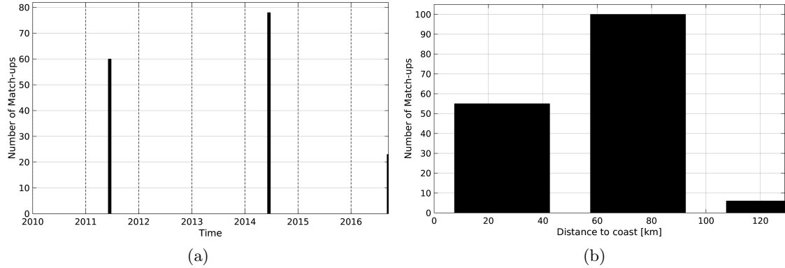
Figure 1: Number of match-ups between TSG-LEGOS-DM and SMOS-L2-DPGS-v662 SSS as a function of time (a) and as function of the distance to coast (b) over the Mediterranean Sea Pi-MEP region and for the full satellite product period.
