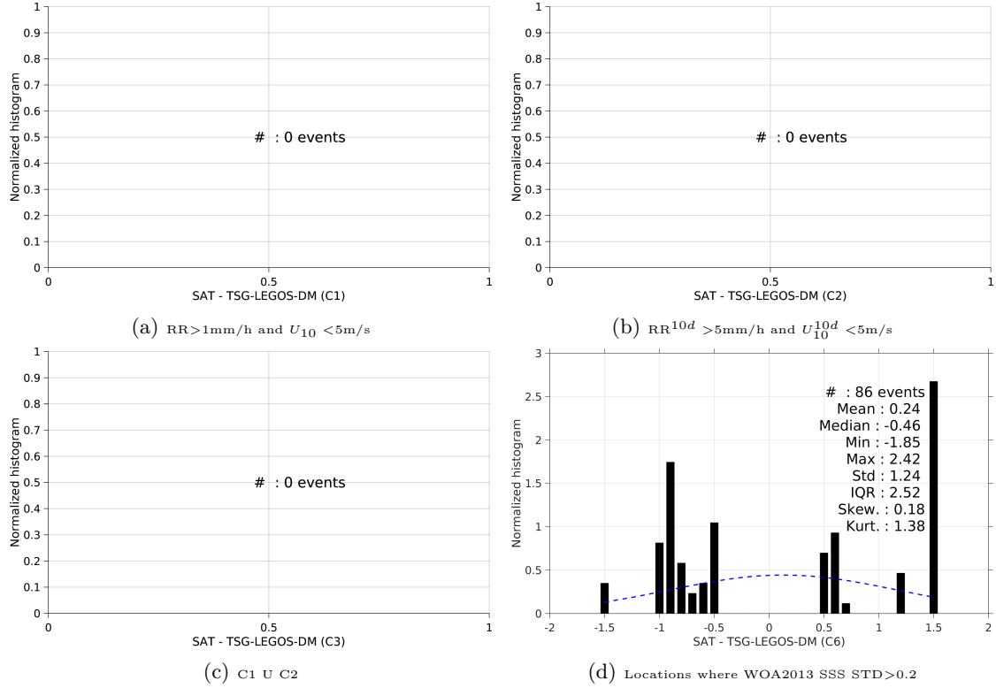
Figure 13: Normalized histogram of \Delta SSS (SMOS-L2-DPGS-v662 - TSG-LEGOS-DM) for 6 different subdatasets corresponding to: RR > 1\text{mm/h} and U_{10} < 5\text{m/s} (a), RR^{10d} > 5\text{mm/h} and U_{10}^{10d} < 5\text{m/s} (b), C1 \cup C2 (c), Locations where WOA2013 SSS STD > 0.2 (d).
