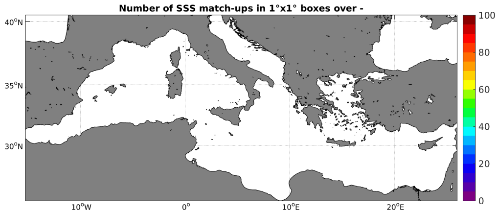
Figure 4: Number of SSS match-ups between TSG-GOSUD-Sailing-ship SSS and the SMOS-L2-DPGS-v662 SSS product for the Mediterranean Sea Pi-MEP region over 1°x1° boxes and for the full satellite product period.
