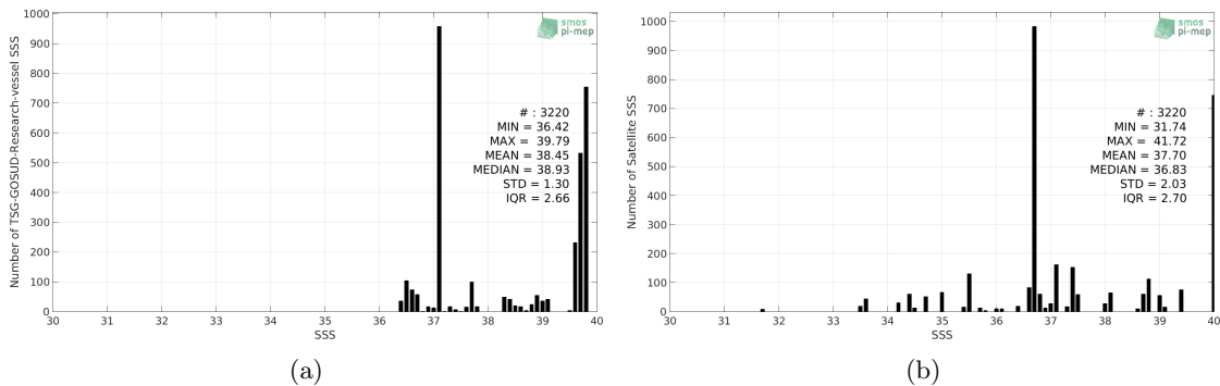
Figure 2: Histograms of SSS from TSG-GOSUD-Research-vessel (a) and SMOS L2 v662 (ESA) (b) considering all match-up pairs per bins of 0.1 over the Mediterranean Sea Pi-MEP region and for the full satellite product period.
