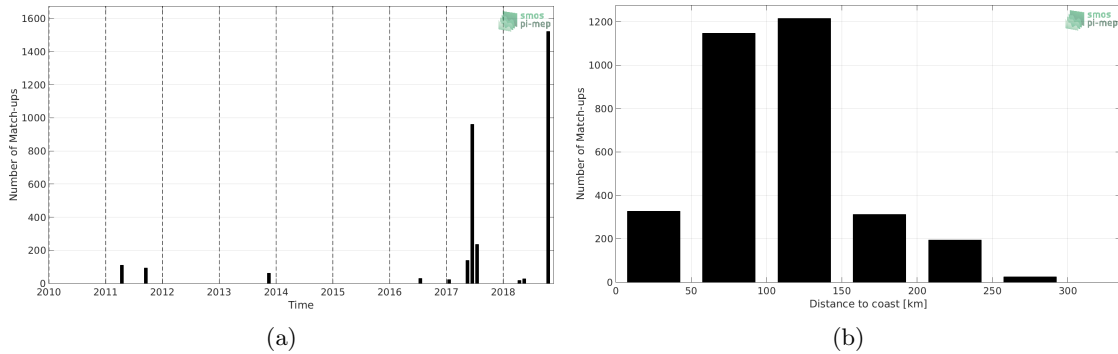
Figure 1: Number of match-ups between TSG-GOSUD-Research-vessel and SMOS L2 v662 (ESA) SSS as a function of time (a) and as function of the distance to coast (b) over the Mediterranean Sea Pi-MEP region and for the full satellite product period.
