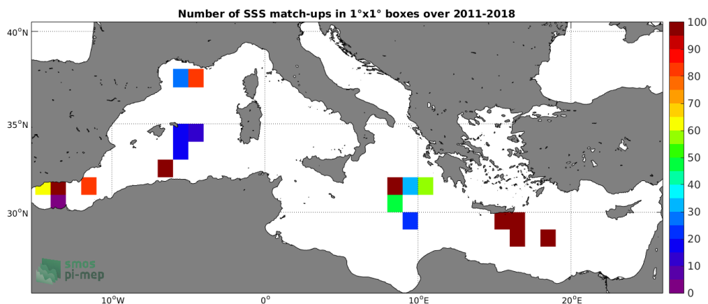
Figure 4: Number of SSS match-ups between TSG-GOSUD-Research-vessel SSS and the SMOS L2 v662 (ESA) SSS product for the Mediterranean Sea Pi-MEP region over 1^\circ \times 1^\circ boxes and for the full satellite product period.
