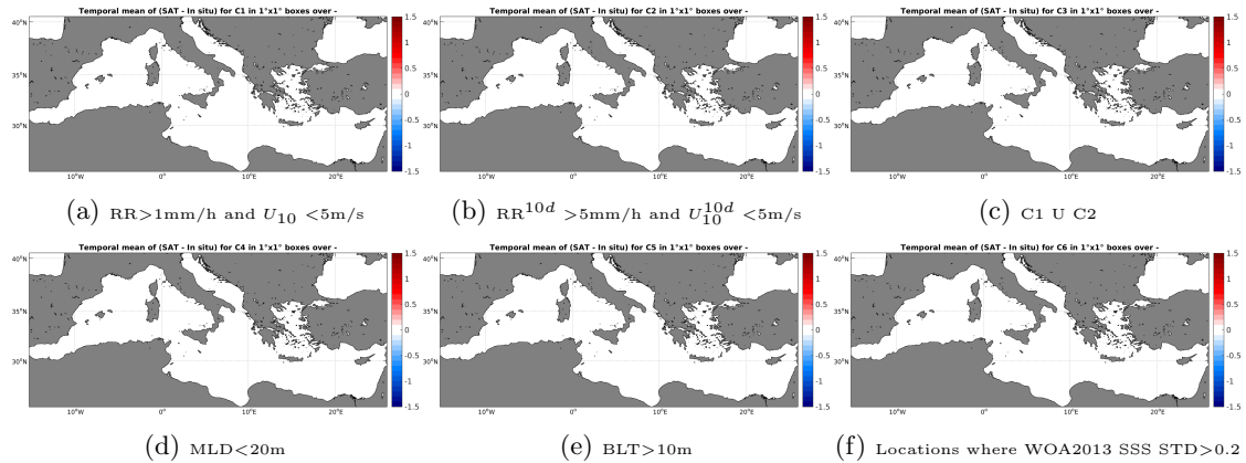
Figure 12: Temporal mean gridded over spatial boxes of size 1^\circ \times 1^\circ of \Delta SSS (SMOS-L2-DPGS-v662 - Sea mammals) for 6 different subdatasets corresponding to:RR >1 mm/h and U_{10} < 5 m/s (a), RR ^{10d} > 5 mm/h and U_{10}^{10d} < 5 m/s (b), C1 U C2 (c),MLD <20 m (d),BLT >10 m (e),Locations where WOA2013 SSS STD >0.2 (f).
