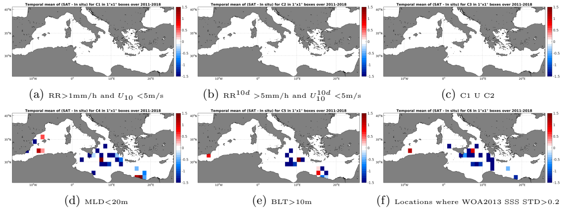
Figure 12: Temporal mean gridded over spatial boxes of size 1^\circ \times 1^\circ of \Delta\text{SSS} (SMOS-L2-DPGS-v662 - Argo) for 6 different subdatasets corresponding to: \text{RR} > 1\text{mm/h} and U_{10} < 5\text{m/s} (a), \text{RR}^{10d} > 5\text{mm/h} and U_{10}^{10d} < 5\text{m/s} (b), C1 U C2 (c), \text{MLD} < 20\text{m} (d), \text{BLT} > 10\text{m} (e), Locations where WOA2013 SSS STD > 0.2 (f).
