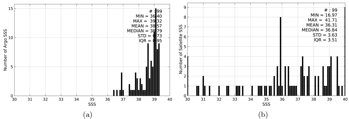
Figure 2: Histograms of SSS from Argo (a) and SMOS-L2-DPGS-v662 (b) considering all match-up pairs per bins of 0.1 over the Mediterranean Sea Pi-MEP region and for the full satellite product period.
