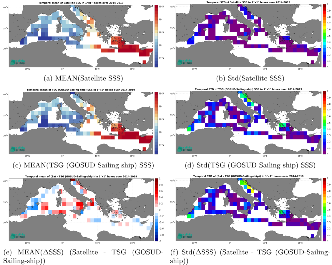
Figure 7: Temporal mean (left) and Std (right) of SSS from SMAP SSS L4 OI v3 - Monthly (ESR) (top), TSG (GOSUD-Sailing-ship) (middle), and of \Delta\text{SSS} (Satellite - TSG (GOSUD-Sailing-ship)). Only match-up pairs are used to generate these maps.
