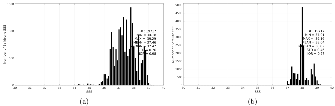
Figure 3: Histograms of SSS from Saildrone (a) and SMAP SSS L4 OI v3 - Monthly (ESR) (b) considering all match-up pairs per bins of 0.1 over the Mediterranean Sea Pi-MEP region and for the full satellite product period.
