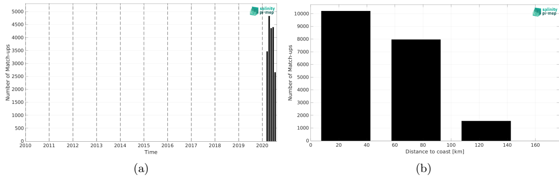
Figure 2: Number of match-ups between Saildrone and SMAP SSS L4 OI v3 - Monthly (ESR) SSS as a function of time (a) and as function of the distance to coast (b) over the Mediterranean Sea Pi-MEP region and for the full satellite product period.
