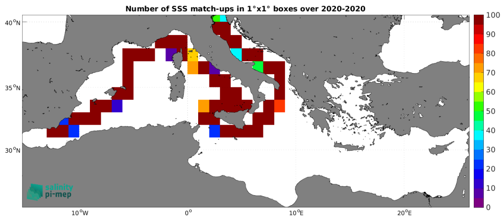
Figure 5: Number of SSS match-ups between Saildrone SSS and the SMAP SSS L4 OI v3 - Monthly (ESR) SSS product for the Mediterranean Sea Pi-MEP region over 1^\circ \times 1^\circ boxes and for the full satellite product period.
