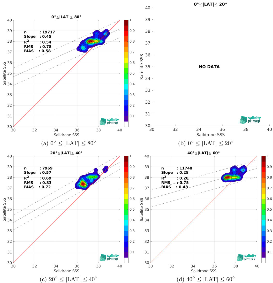
Figure 10: Contour maps of the concentration of SMAP SSS L4 OI v3 - Monthly (ESR) SSS (y-axis) versus Saildrone SSS (x-axis) at match-up pairs for different latitude bands. For each plot, the red line shows x=y . The black thin and dashed lines indicate a linear fit through the data cloud and the \pm 95\% confidence levels, respectively. The number match-up pairs n , the slope and R^2 coefficient of the linear fit, the root mean square (RMS) and the mean bias between satellite and in situ data are indicated for each latitude band in each plots.
