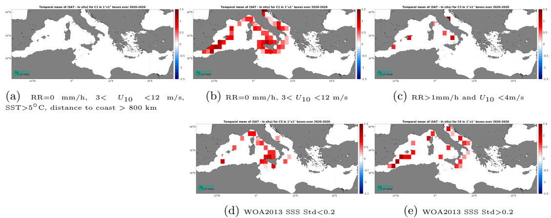
Figure 14: Temporal mean gridded over spatial boxes of size 1^\circ \times 1^\circ of \Delta SSS (SMAP SSS L4 OI v3 - Monthly (ESR) - Saildrone) for 5 different subdatasets corresponding to:RR=0 mm/h, 3 < U_{10} < 12 m/s, SST>5°C, distance to coast > 800 km (a), RR=0 mm/h, 3 < U_{10} < 12 m/s (b), RR>1mm/h and U_{10} < 4 m/s (c), WOA2013 SSS Std<0.2 (d), WOA2013 SSS Std>0.2 (e).
