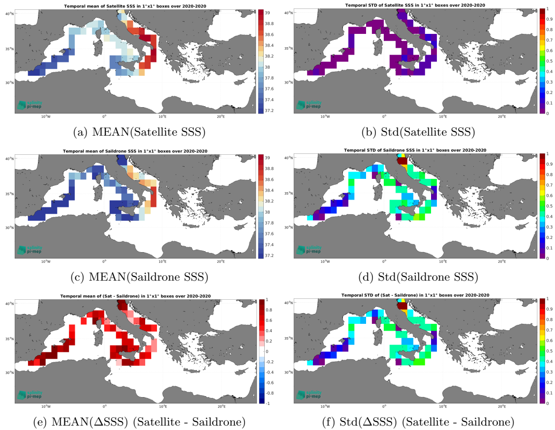
Figure 7: Temporal mean (left) and Std (right) of SSS from SMAP SSS L4 OI v3 - Monthly (ESR) (top), Saildrone (middle), and of \Delta SSS (Satellite - Saildrone). Only match-up pairs are used to generate these maps.
