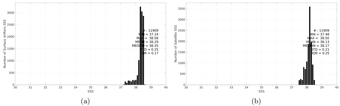
Figure 3: Histograms of SSS from Surface drifters (a) and SMAP SSS L4 OI v3 - Monthly (ESR) (b) considering all match-up pairs per bins of 0.1 over the Mediterranean Sea Pi-MEP region and for the full satellite product period.
