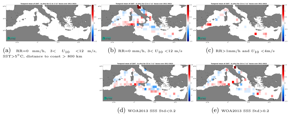
Figure 14: Temporal mean gridded over spatial boxes of size 1^\circ \times 1^\circ of \Delta\text{SSS} (SMAP SSS L4 OI v3 - Daily (ESR) - TSG (LEGOS-DM)) for 5 different subdatasets corresponding to:RR=0 mm/h, 3 < U_{10} < 12 m/s, SST>5°C, distance to coast > 800 km (a), RR=0 mm/h, 3 < U_{10} < 12 m/s (b), RR>1mm/h and U_{10} < 4 m/s (c), WOA2013 SSS Std<0.2 (d), WOA2013 SSS Std>0.2 (e).
