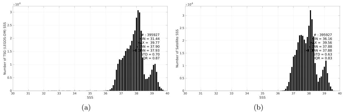
Figure 3: Histograms of SSS from TSG (LEGOS-DM) (a) and SMAP SSS L4 OI v3 - Daily (ESR) (b) considering all match-up pairs per bins of 0.1 over the Mediterranean Sea Pi-MEP region and for the full satellite product period.
