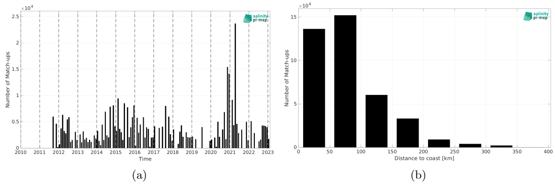
Figure 2: Number of match-ups between TSG (LEGOS-DM) and SMAP SSS L4 OI v3 - Daily (ESR) SSS as a function of time (a) and as function of the distance to coast (b) over the Mediterranean Sea Pi-MEP region and for the full satellite product period.
