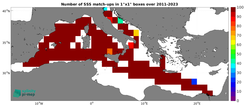
Figure 5: Number of SSS match-ups between TSG (LEGOS-DM) SSS and the SMAP SSS L4 OI v3 - Daily (ESR) SSS product for the Mediterranean Sea Pi-MEP region over 1^\circ \times 1^\circ boxes and for the full satellite product period.
