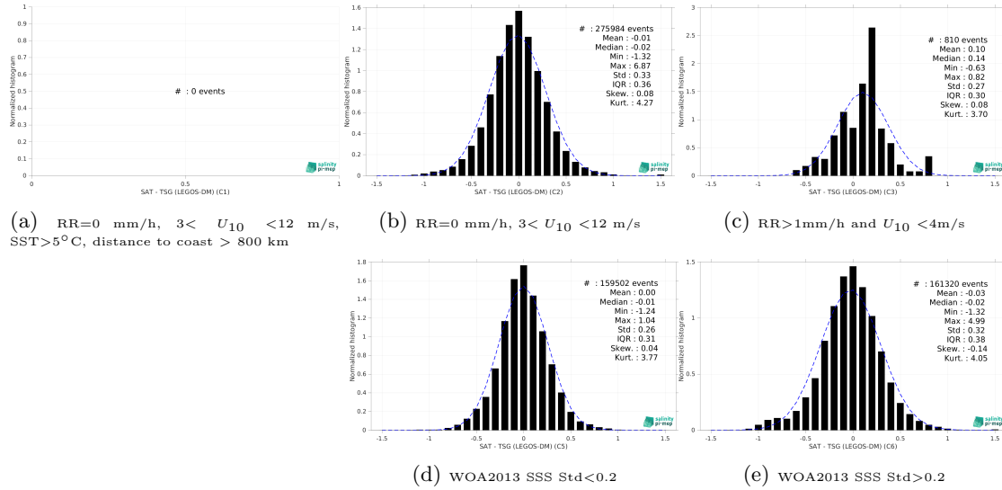
Figure 15: Normalized histogram of \Delta SSS (SMAP SSS L4 OI v3 - Daily (ESR) - TSG (LEGOS-DM)) for 5 different subdatasets corresponding to: RR=0 mm/h, 3 < U_{10} < 12 m/s, SST > 5°C, distance to coast > 800 km (a), RR=0 mm/h, 3 < U_{10} < 12 m/s (b), RR > 1mm/h and U_{10} < 4 m/s (c), WOA2013 SSS Std < 0.2 (d), WOA2013 SSS Std > 0.2 (e).
