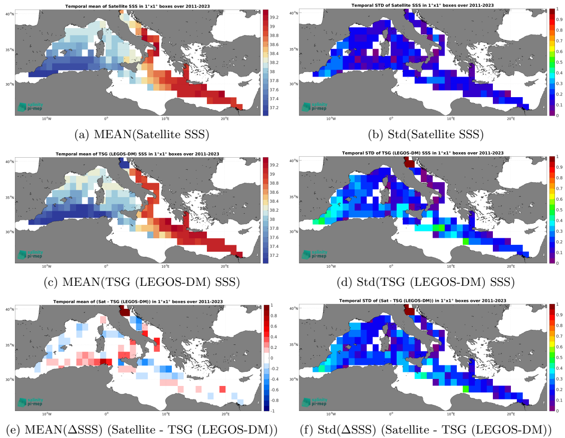
Figure 7: Temporal mean (left) and Std (right) of SSS from SMAP SSS L4 OI v3 - Daily (ESR) (top), TSG (LEGOS-DM) (middle), and of \Delta SSS (Satellite - TSG (LEGOS-DM)). Only match-up pairs are used to generate these maps.
