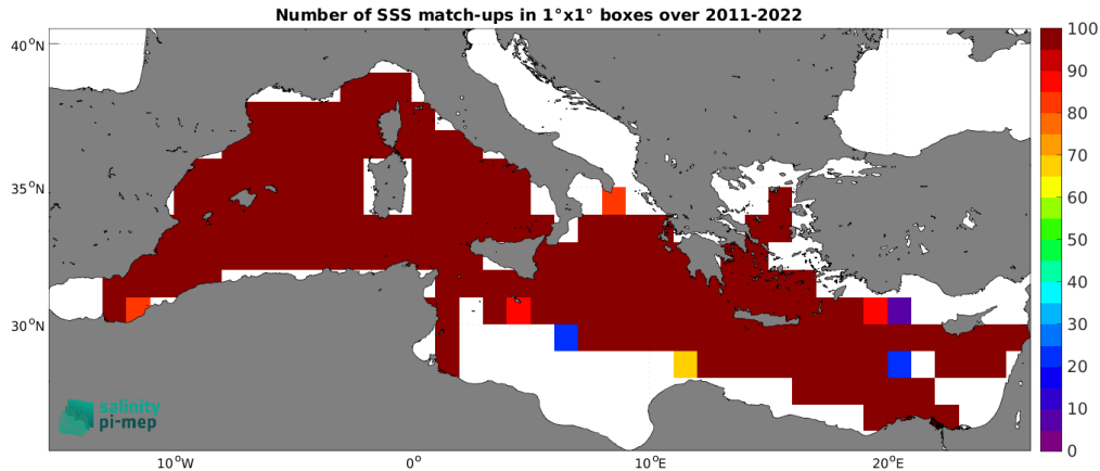
Figure 5: Number of SSS match-ups between TSG (GOSUD-Research-vessel) SSS and the SMAP SSS L4 OI v3 - Daily (ESR) SSS product for the Mediterranean Sea Pi-MEP region over 1^\circ \times 1^\circ boxes and for the full satellite product period.
