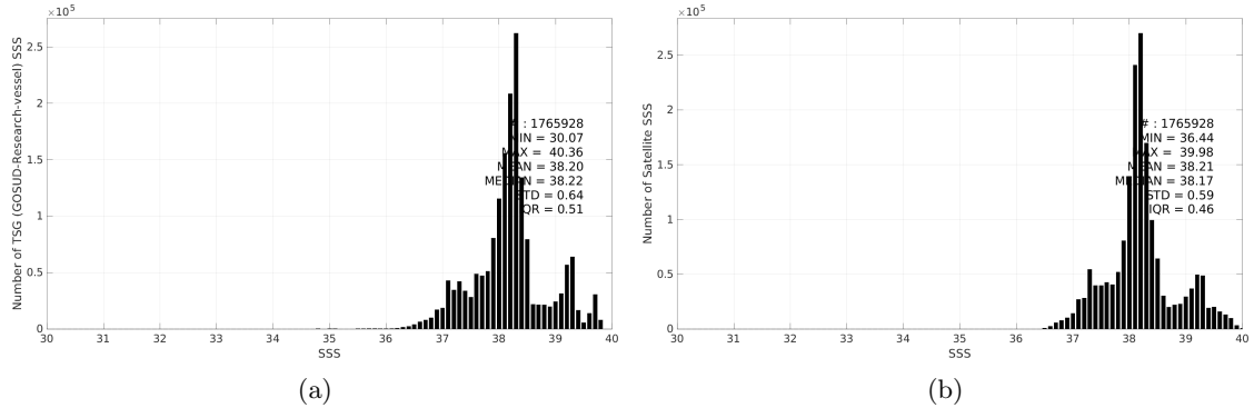
Figure 3: Histograms of SSS from TSG (GOSUD-Research-vessel) (a) and SMAP SSS L4 OI v3 - Daily (ESR) (b) considering all match-up pairs per bins of 0.1 over the Mediterranean Sea Pi-MEP region and for the full satellite product period.
