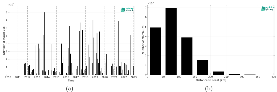
Figure 2: Number of match-ups between TSG (GOSUD-Research-vessel) and SMAP SSS L4 OI v3 - Daily (ESR) SSS as a function of time (a) and as function of the distance to coast (b) over the Mediterranean Sea Pi-MEP region and for the full satellite product period.
