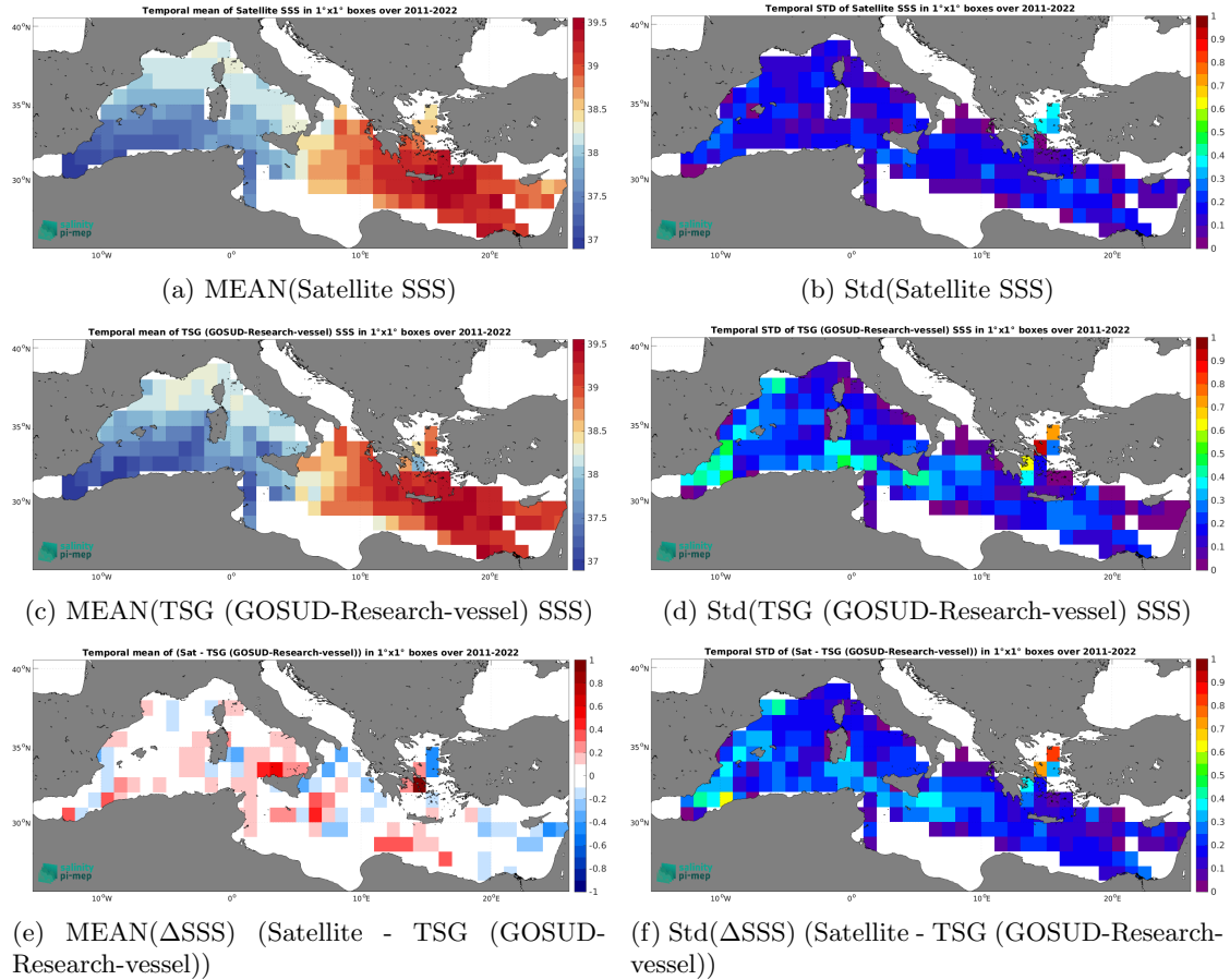
Figure 7: Temporal mean (left) and Std (right) of SSS from SMAP SSS L4 OI v3 - Daily (ESR) (top), TSG (GOSUD-Research-vessel) (middle), and of \Delta\text{SSS} (Satellite - TSG (GOSUD-Research-vessel)). Only match-up pairs are used to generate these maps.
