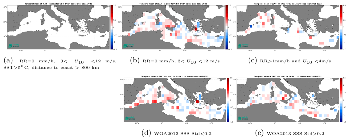
Figure 14: Temporal mean gridded over spatial boxes of size 1^\circ \times 1^\circ of \Delta SSS (SMAP SSS L4 OI v3 - Daily (ESR) - TSG (GOSUD-Research-vessel)) for 5 different subdatasets corresponding to:RR=0 mm/h, 3 < U_{10} < 12 m/s, SST>5°C, distance to coast > 800 km (a), RR=0 mm/h, 3 < U_{10} < 12 m/s (b), RR>1mm/h and U_{10} < 4 m/s (c), WOA2013 SSS Std<0.2 (d), WOA2013 SSS Std>0.2 (e).
