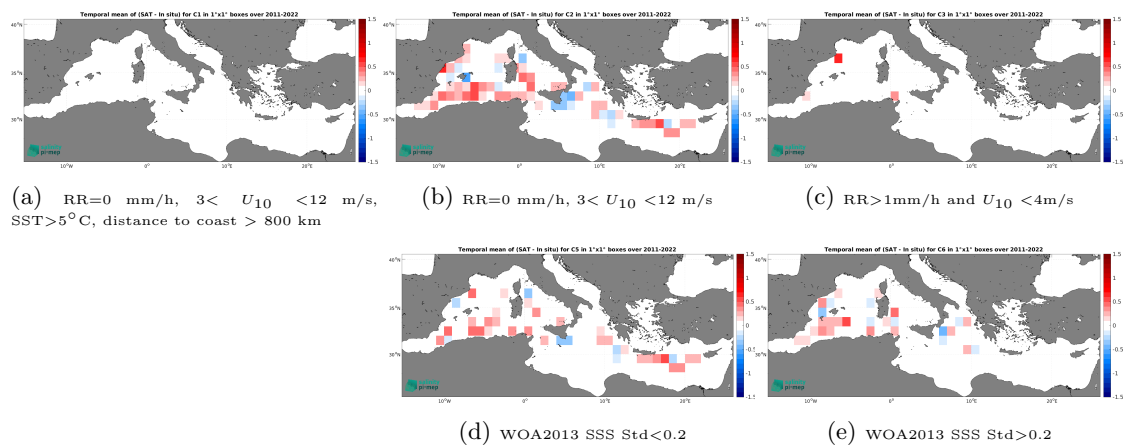
Figure 14: Temporal mean gridded over spatial boxes of size 1^\circ \times 1^\circ of \Delta SSS (SMAP SSS L4 OI v3 - Daily (ESR) - TSG (CSIC-UTM)) for 5 different subdatasets corresponding to:RR=0 mm/h, 3 < U_{10} < 12 m/s, SST>5°C, distance to coast > 800 km (a), RR=0 mm/h, 3 < U_{10} < 12 m/s (b), RR>1mm/h and U_{10} < 4 m/s (c), WOA2013 SSS Std<0.2 (d), WOA2013 SSS Std>0.2 (e).
