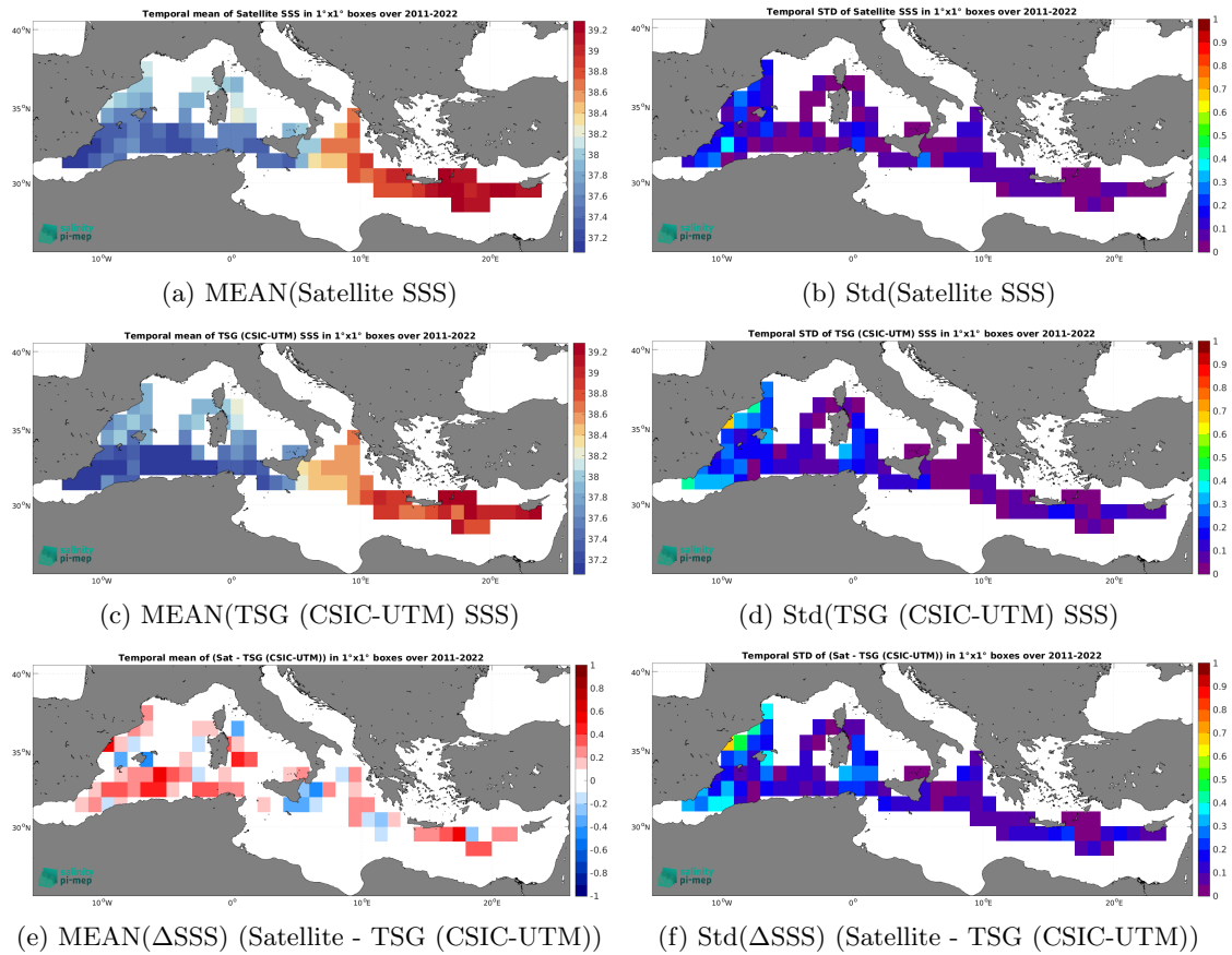
Figure 7: Temporal mean (left) and Std (right) of SSS from SMAP SSS L4 OI v3 - Daily (ESR) (top), TSG (CSIC-UTM) (middle), and of \Delta SSS (Satellite - TSG (CSIC-UTM)). Only match-up pairs are used to generate these maps.
