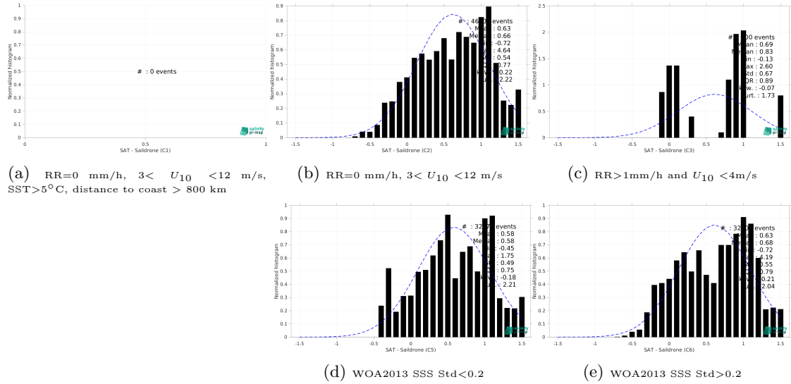
Figure 15: Normalized histogram of \Delta\text{SSS} (SMAP SSS L4 OI v3 - Daily (ESR) - Saildrone) for 5 different subdatasets corresponding to: RR=0 mm/h, 3 < U_{10} < 12 m/s, SST > 5^\circ\text{C} , distance to coast > 800 km (a), RR=0 mm/h, 3 < U_{10} < 12 m/s (b), RR > 1\text{mm/h} and U_{10} < 4\text{m/s} (c), WOA2013 SSS Std < 0.2 (d), WOA2013 SSS Std > 0.2 (e).
