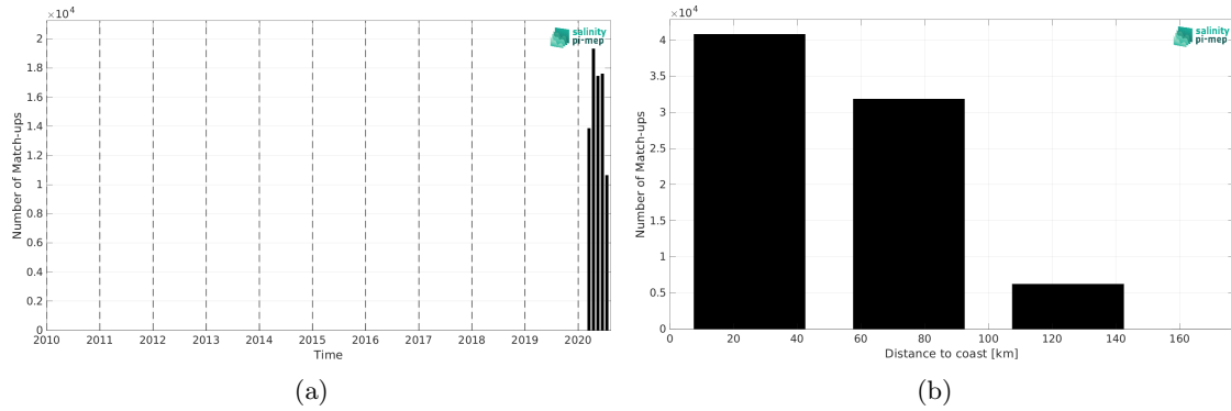
Figure 2: Number of match-ups between Saildrone and SMAP SSS L4 OI v3 - Daily (ESR) SSS as a function of time (a) and as function of the distance to coast (b) over the Mediterranean Sea Pi-MEP region and for the full satellite product period.
