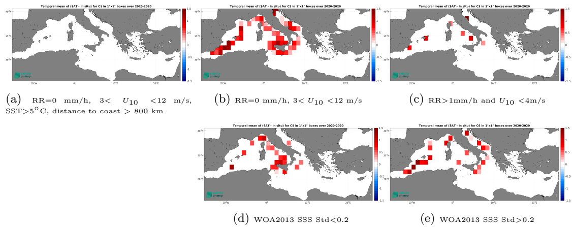
Figure 14: Temporal mean gridded over spatial boxes of size 1^\circ \times 1^\circ of \Delta SSS (SMAP SSS L4 OI v3 - Daily (ESR) - Saildrone) for 5 different subdatasets corresponding to:RR=0 mm/h, 3 < U_{10} < 12 m/s, SST>5°C, distance to coast > 800 km (a), RR=0 mm/h, 3 < U_{10} < 12 m/s (b), RR>1mm/h and U_{10} < 4 m/s (c), WOA2013 SSS Std<0.2 (d), WOA2013 SSS Std>0.2 (e).
