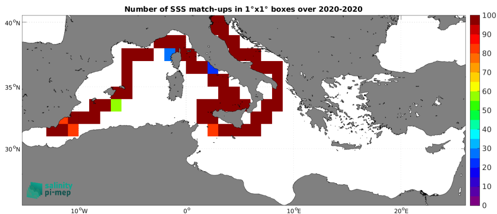
Figure 5: Number of SSS match-ups between Saildrone SSS and the SMAP SSS L4 OI v3 - Daily (ESR) SSS product for the Mediterranean Sea Pi-MEP region over 1^\circ \times 1^\circ boxes and for the full satellite product period.
