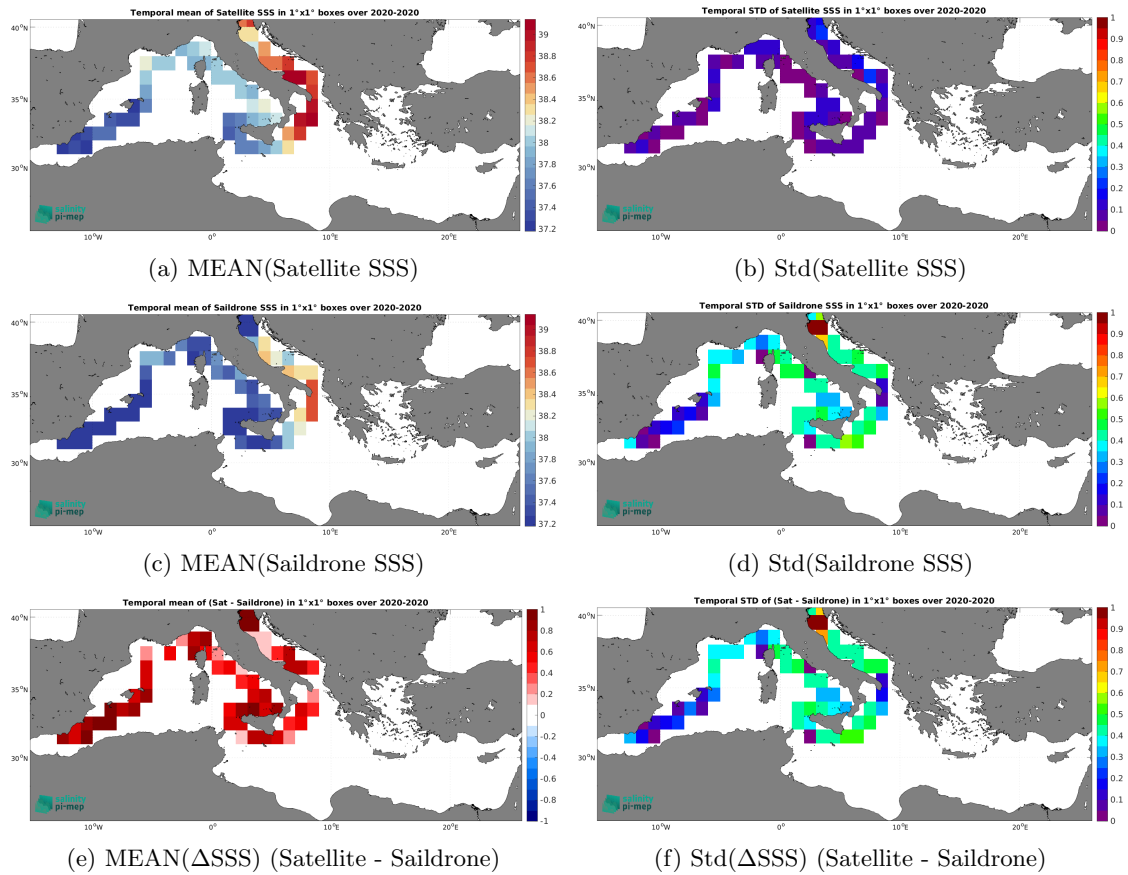
Figure 7: Temporal mean (left) and Std (right) of SSS from SMAP SSS L4 OI v3 - Daily (ESR) (top), Saildrone (middle), and of \Delta SSS (Satellite - Saildrone). Only match-up pairs are used to generate these maps.
