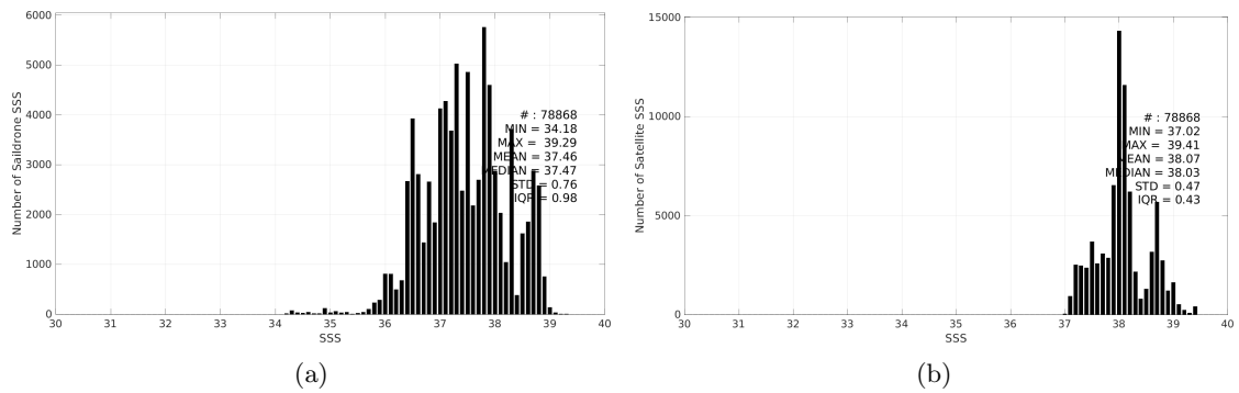
Figure 3: Histograms of SSS from Saildrone (a) and SMAP SSS L4 OI v3 - Daily (ESR) (b) considering all match-up pairs per bins of 0.1 over the Mediterranean Sea Pi-MEP region and for the full satellite product period.
