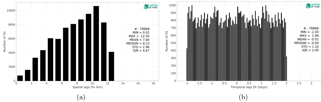
Figure 6: Histograms of the spatial (a) and temporal (b) lags between the location/time of the Sairdrone measurement and the date of the corresponding SMAP SSS L4 OI v3 - Daily (ESR) SSS pixel.
