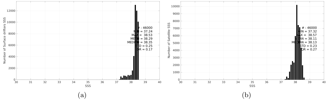
Figure 3: Histograms of SSS from Surface drifters (a) and SMAP SSS L4 OI v3 - Daily (ESR) (b) considering all match-up pairs per bins of 0.1 over the Mediterranean Sea Pi-MEP region and for the full satellite product period.
