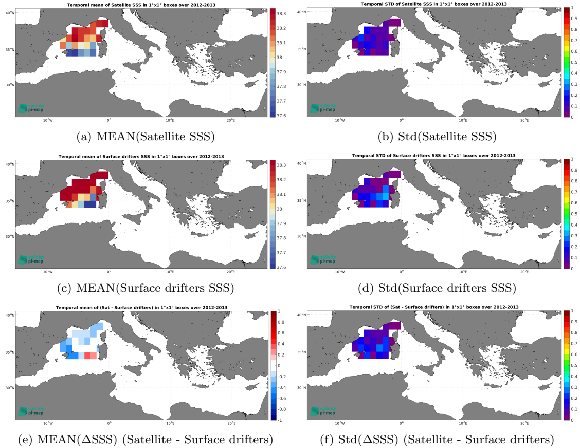
Figure 6: Temporal mean (left) and Std (right) of SSS from SMAP SSS L4 OI v3 - Daily (ESR) (top), Surface drifters (middle), and of \Delta SSS (Satellite - Surface drifters). Only match-up pairs are used to generate these maps.
