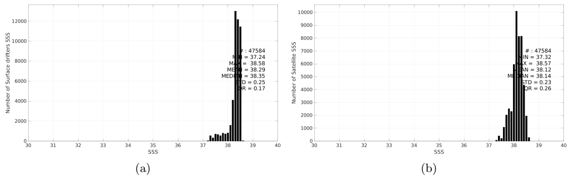
Figure 3: Histograms of SSS from Surface drifters (a) and SMAP SSS L4 OI v3 - Daily (ESR) (b) considering all match-up pairs per bins of 0.1 over the Mediterranean Sea Pi-MEP region and for the full satellite product period.
