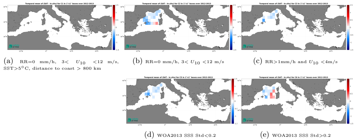
Figure 13: Temporal mean gridded over spatial boxes of size 1^\circ \times 1^\circ of \Delta SSS (SMAP SSS L4 OI v3 - Daily (ESR) - Surface drifters) for 5 different subdatasets corresponding to:RR=0 mm/h, 3 < U_{10} < 12 m/s, SST >5^\circ\text{C} , distance to coast > 800 km (a), RR=0 mm/h, 3 < U_{10} < 12 m/s (b), RR >1 mm/h and U_{10} < 4 m/s (c), WOA2013 SSS Std <0.2 (d), WOA2013 SSS Std >0.2 (e).
