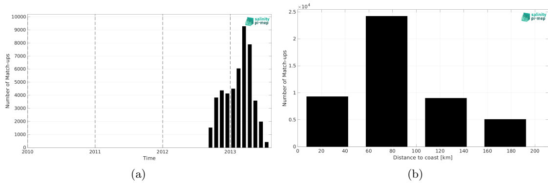
Figure 2: Number of match-ups between Surface drifters and SMAP SSS L4 OI v3 - Daily (ESR) SSS as a function of time (a) and as function of the distance to coast (b) over the Mediterranean Sea Pi-MEP region and for the full satellite product period.
