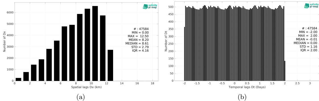
Figure 5: Histograms of the spatial (a) and temporal (b) lags between the location/time of the Surface drifters measurement and the date of the corresponding SMAP SSS L4 OI v3 - Daily (ESR) SSS pixel.
