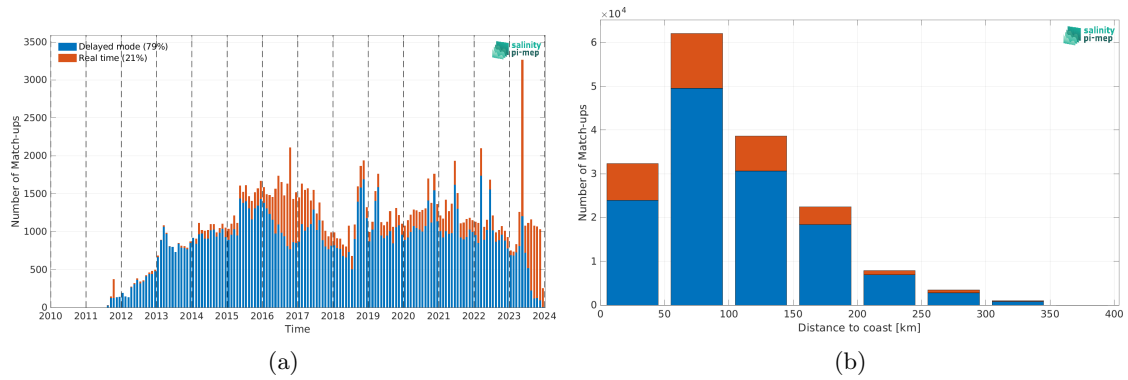
Figure 2: Number of match-ups between Argo and SMAP SSS L4 OI v3 - Daily (ESR) SSS as a function of time (a) and as function of the distance to coast (b) over the Mediterranean Sea Pi-MEP region and for the full satellite product period.
