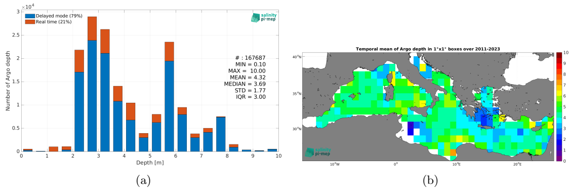
Figure 4: Histograms of the depth of the upper level SSS measurements from Argo in the Match-up DataBase for the Mediterranean Sea Pi-MEP region (a) and temporal mean spatial distribution of pressure of the in situ SSS data over 1^\circ \times 1^\circ boxes and for the full satellite product period (b).
