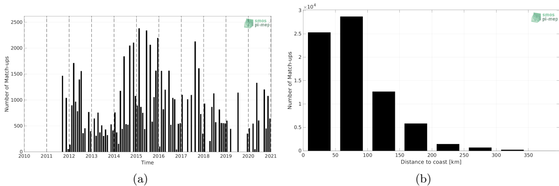
Figure 1: Number of match-ups between TSG (LEGOS-DM) and SMAP SSS L4 OI v2 - 7 Days (ESR) SSS as a function of time (a) and as function of the distance to coast (b) over the Mediterranean Sea Pi-MEP region and for the full satellite product period.
