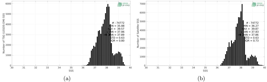
Figure 2: Histograms of SSS from TSG (LEGOS-DM) (a) and SMAP SSS L4 OI v2 - 7 Days (ESR) (b) considering all match-up pairs per bins of 0.1 over the Mediterranean Sea Pi-MEP region and for the full satellite product period.
