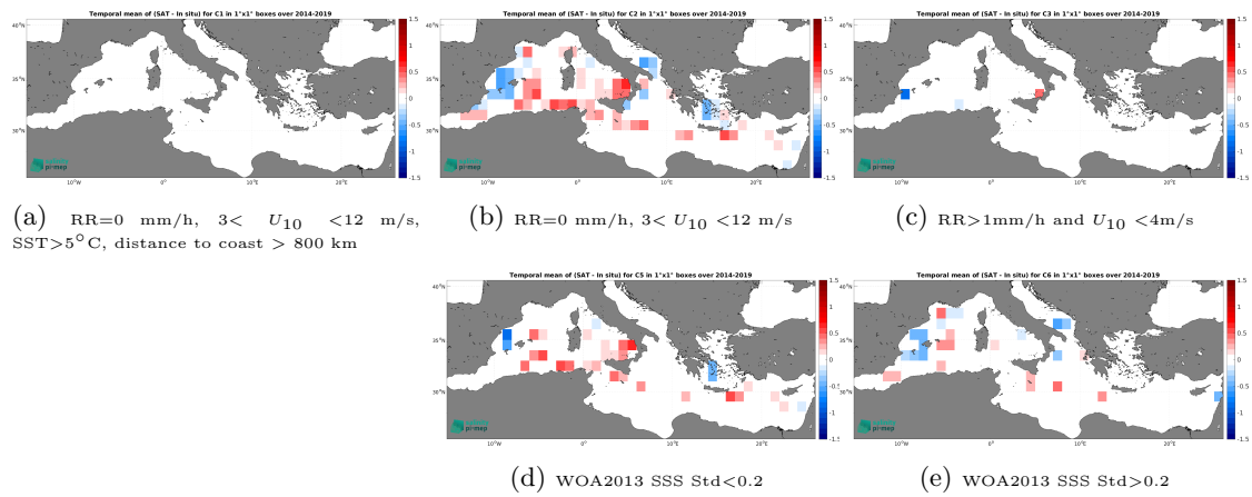
Figure 12: Temporal mean gridded over spatial boxes of size 1^\circ \times 1^\circ of \Delta\text{SSS} (SMAP SSS L4 OI v2 - 7 Days (ESR) - TSG (GOSUD-Sailing-ship)) for 5 different subdatasets corresponding to:RR=0 mm/h, 3 < U_{10} < 12 m/s, SST>5°C, distance to coast > 800 km (a), RR=0 mm/h, 3 < U_{10} < 12 m/s (b), RR>1mm/h and U_{10} < 4 m/s (c), WOA2013 SSS Std<0.2 (d), WOA2013 SSS Std>0.2 (e).
