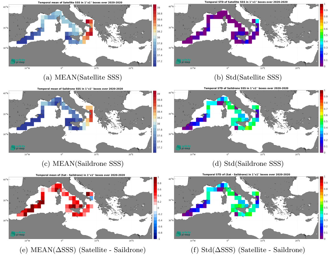
Figure 6: Temporal mean (left) and Std (right) of SSS from SMAP SSS L4 OI v2 - 7 Days (ESR) (top), Sairdrone (middle), and of \Delta SSS (Satellite - Sairdrone). Only match-up pairs are used to generate these maps.
