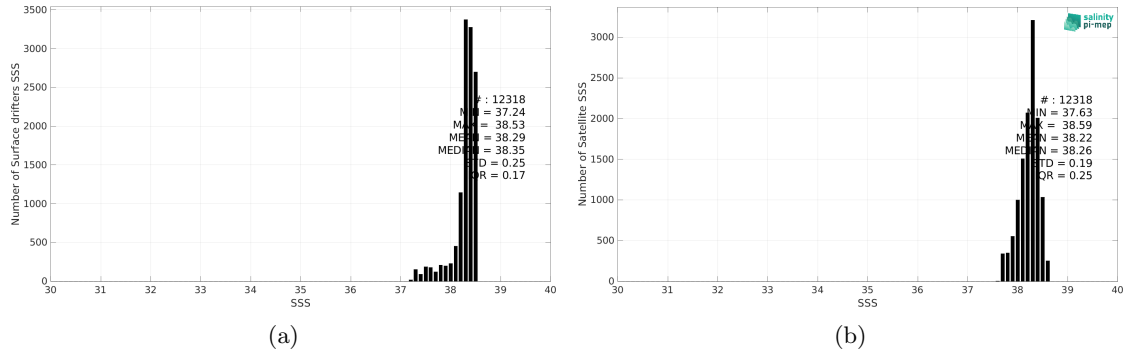
Figure 2: Histograms of SSS from Surface drifters (a) and SMAP SSS L4 OI v2 - 7 Days (ESR) (b) considering all match-up pairs per bins of 0.1 over the Mediterranean Sea Pi-MEP region and for the full satellite product period.
