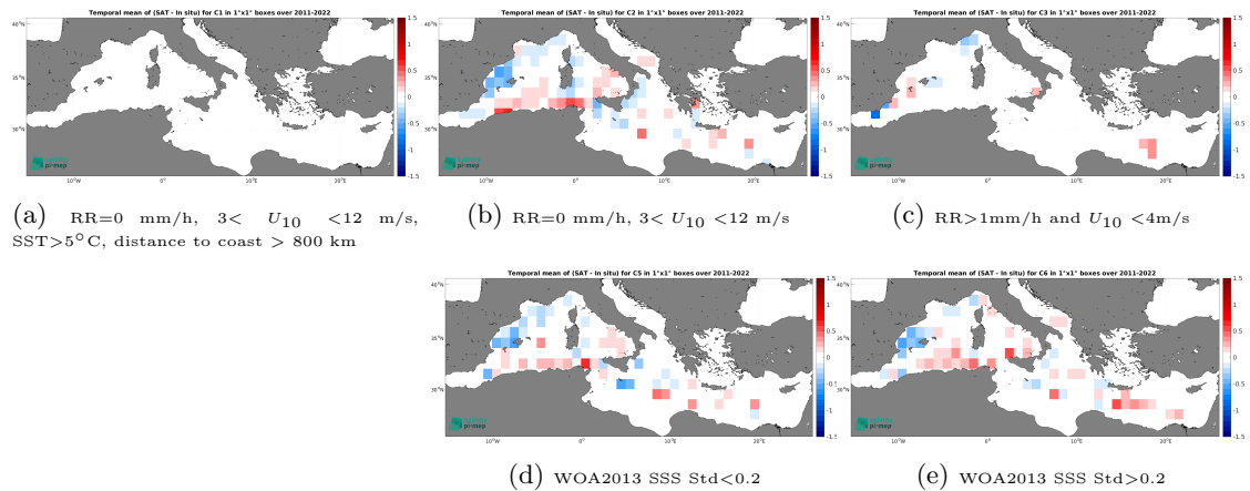
Figure 12: Temporal mean gridded over spatial boxes of size 1^\circ \times 1^\circ of \Delta SSS (SMAP SSS L4 OI v2 - Monthly (IPRC) - TSG (LEGOS-DM)) for 5 different subdatasets corresponding to:RR=0 mm/h, 3 < U_{10} < 12 m/s, SST >5^\circ\text{C} , distance to coast > 800 km (a), RR=0 mm/h, 3 < U_{10} < 12 m/s (b), RR >1 mm/h and U_{10} < 4 m/s (c), WOA2013 SSS Std <0.2 (d), WOA2013 SSS Std >0.2 (e).
