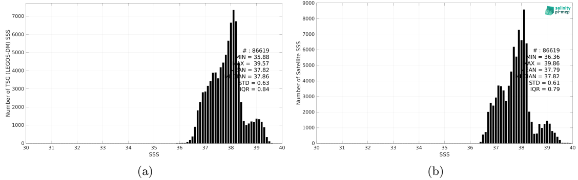
Figure 2: Histograms of SSS from TSG (LEGOS-DM) (a) and SMAP SSS L4 OI v2 - Monthly (IPRC) (b) considering all match-up pairs per bins of 0.1 over the Mediterranean Sea Pi-MEP region and for the full satellite product period.
