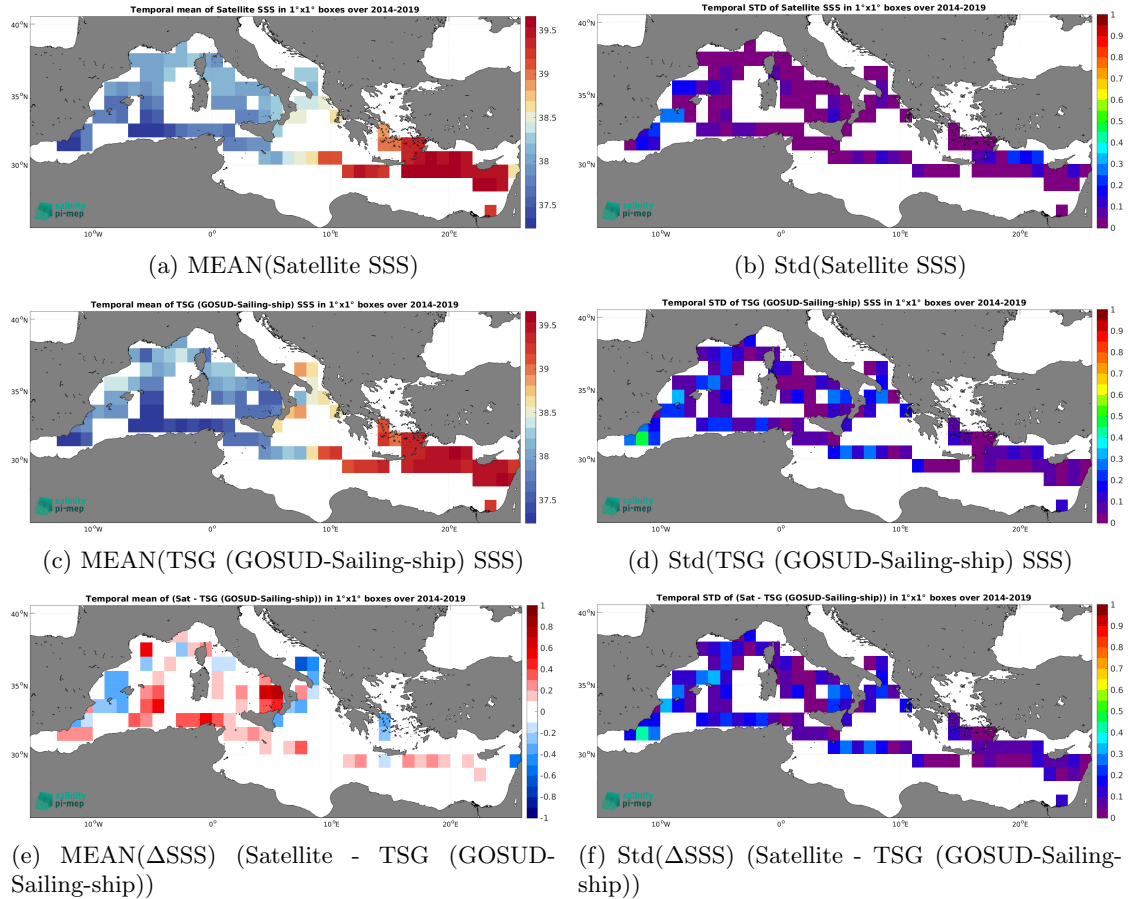
Figure 6: Temporal mean (left) and Std (right) of SSS from SMAP SSS L4 OI v2 - Monthly (IPRC) (top), TSG (GOSUD-Sailing-ship) ( in situ ) (middle), and of \Delta\text{SSS} (Satellite - TSG (GOSUD-Sailing-ship)). Only match-up pairs are used to generate these maps.
