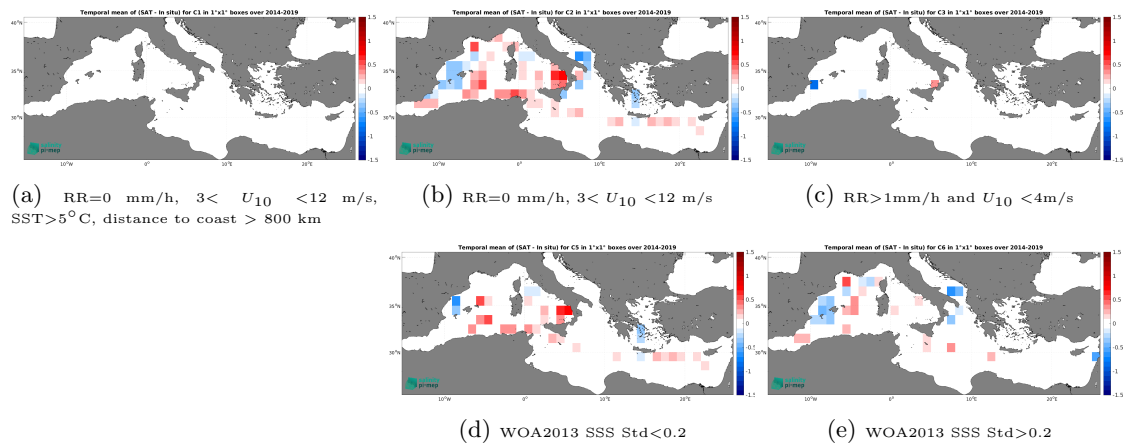
Figure 12: Temporal mean gridded over spatial boxes of size 1^\circ \times 1^\circ of \Delta\text{SSS} (SMAP SSS L4 OI v2 - Monthly (IPRC) - TSG (GOSUD-Sailing-ship)) for 5 different subdatasets corresponding to:RR=0 mm/h, 3 < U_{10} < 12 m/s, SST>5°C, distance to coast > 800 km (a), RR=0 mm/h, 3 < U_{10} < 12 m/s (b), RR>1mm/h and U_{10} < 4 m/s (c), WOA2013 SSS Std<0.2 (d), WOA2013 SSS Std>0.2 (e).
