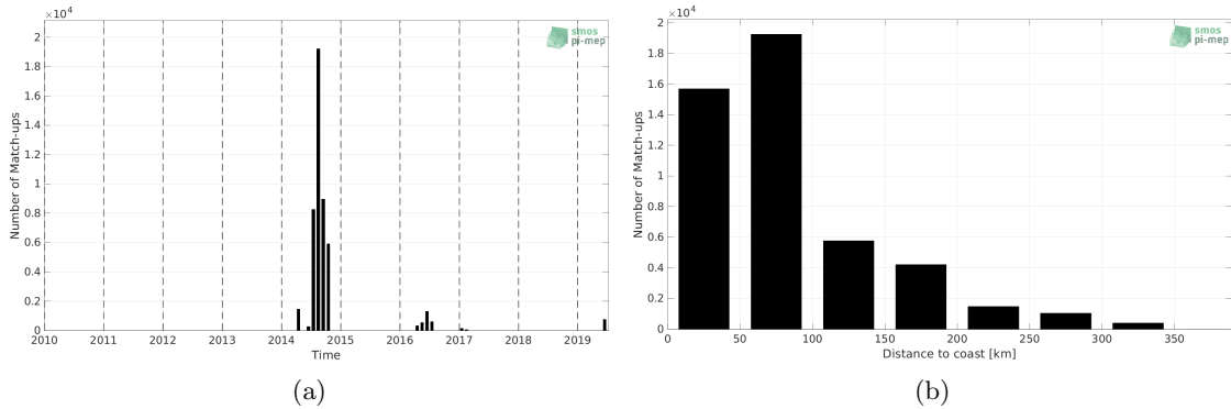
Figure 1: Number of match-ups between TSG (GOSUD-Sailing-ship) and SMAP SSS L4 OI v2 - Monthly (IPRC) SSS as a function of time (a) and as function of the distance to coast (b) over the Mediterranean Sea Pi-MEP region and for the full satellite product period.
