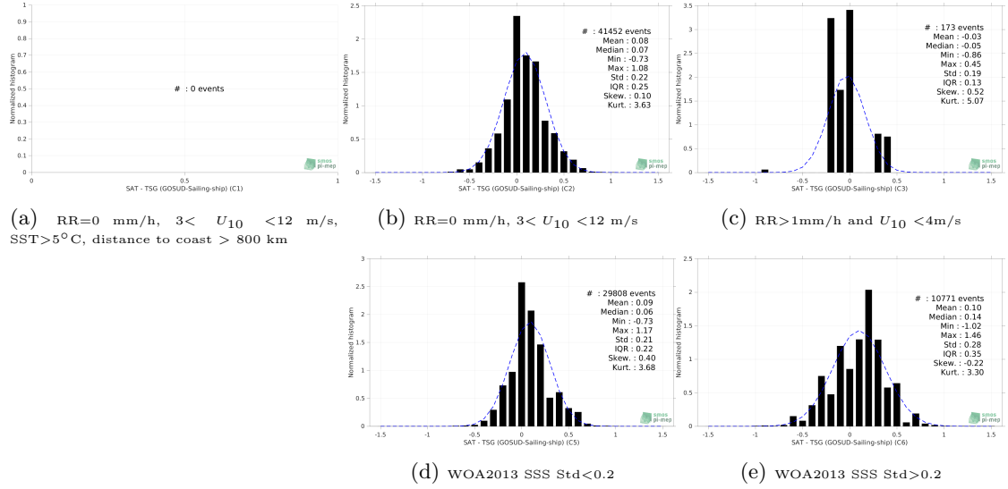
Figure 13: Normalized histogram of \Delta SSS (SMAP SSS L4 OI v2 - Monthly (IPRC) - TSG (GOSUD-Sailing-ship)) for 5 different subdatasets corresponding to: RR=0 mm/h, 3 < U_{10} < 12 m/s, SST > 5°C, distance to coast > 800 km (a), RR=0 mm/h, 3 < U_{10} < 12 m/s (b), RR > 1mm/h and U_{10} < 4 m/s (c), WOA2013 SSS Std < 0.2 (d), WOA2013 SSS Std > 0.2 (e).
