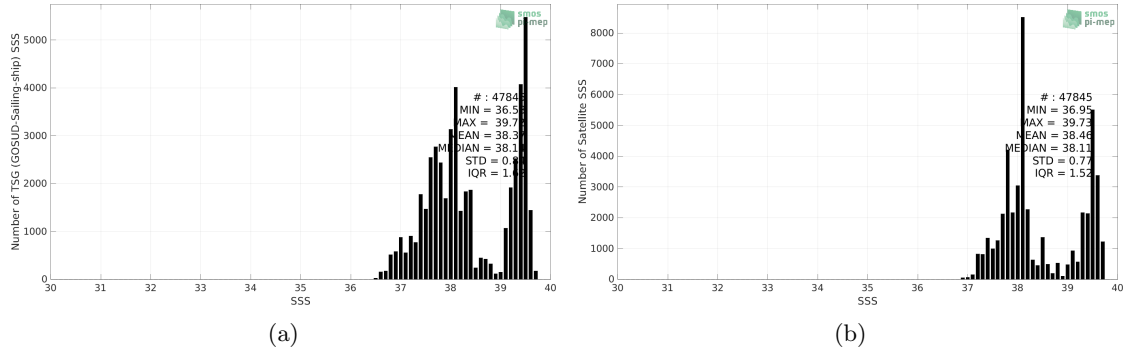
Figure 2: Histograms of SSS from TSG (GOSUD-Sailing-ship) (a) and SMAP SSS L4 OI v2 - Monthly (IPRC) (b) considering all match-up pairs per bins of 0.1 over the Mediterranean Sea Pi-MEP region and for the full satellite product period.
