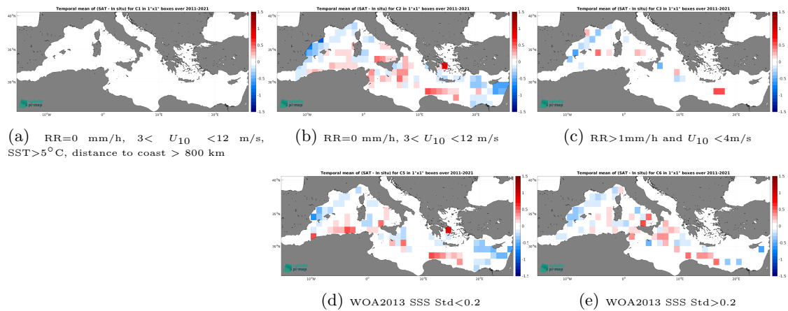
Figure 12: Temporal mean gridded over spatial boxes of size 1^\circ \times 1^\circ of \Delta\text{SSS} (SMAP SSS L4 OI v2 - Monthly (IPRC) - TSG (GOSUD-Research-vessel)) for 5 different subdatasets corresponding to:RR=0 mm/h, 3 < U_{10} < 12 m/s, SST>5°C, distance to coast > 800 km (a), RR=0 mm/h, 3 < U_{10} < 12 m/s (b), RR>1mm/h and U_{10} < 4 m/s (c), WOA2013 SSS Std<0.2 (d), WOA2013 SSS Std>0.2 (e).
