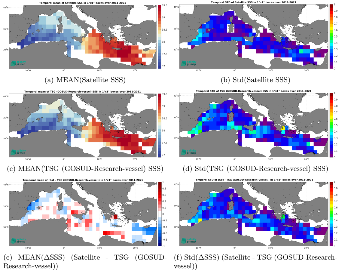
Figure 6: Temporal mean (left) and Std (right) of SSS from SMAP SSS L4 OI v2 - Monthly (IPRC) (top), TSG (GOSUD-Research-vessel) (middle), and of \Delta\text{SSS} (Satellite - TSG (GOSUD-Research-vessel)). Only match-up pairs are used to generate these maps.
