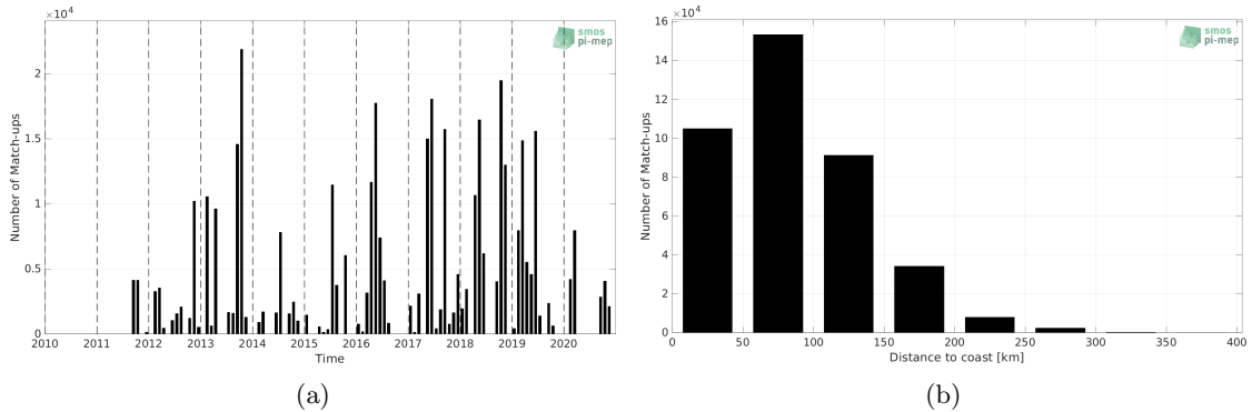
Figure 1: Number of match-ups between TSG (GOSUD-Research-vessel) and SMAP SSS L4 OI v2 - Monthly (IPRC) SSS as a function of time (a) and as function of the distance to coast (b) over the Mediterranean Sea Pi-MEP region and for the full satellite product period.
