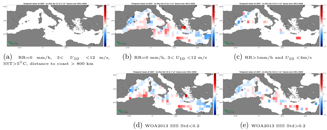
Figure 12: Temporal mean gridded over spatial boxes of size 1^\circ \times 1^\circ of \Delta SSS (SMAP SSS L4 OI v2 - Monthly (IPRC) - TSG (GOSUD-Research-vessel)) for 5 different subdatasets corresponding to:RR=0 mm/h, 3 < U_{10} < 12 m/s, SST>5°C, distance to coast > 800 km (a), RR=0 mm/h, 3 < U_{10} < 12 m/s (b), RR>1mm/h and U_{10} < 4 m/s (c), WOA2013 SSS Std<0.2 (d), WOA2013 SSS Std>0.2 (e).
