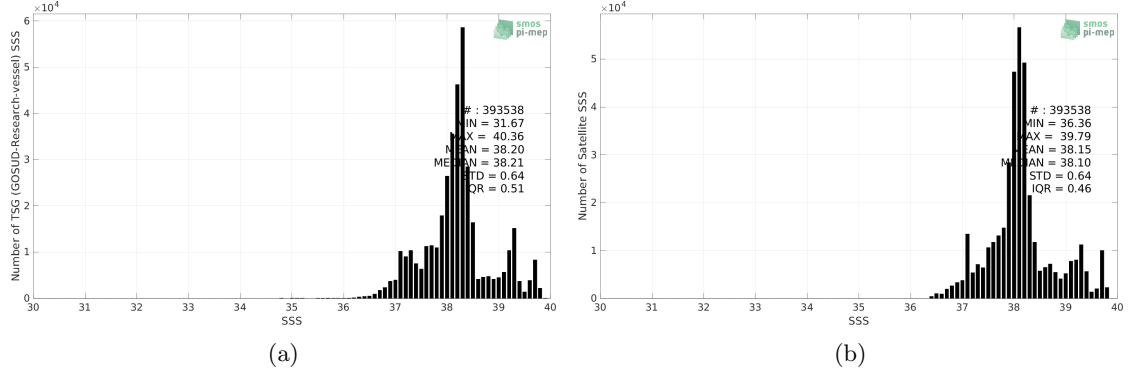
Figure 2: Histograms of SSS from TSG (GOSUD-Research-vessel) (a) and SMAP SSS L4 OI v2 - Monthly (IPRC) (b) considering all match-up pairs per bins of 0.1 over the Mediterranean Sea Pi-MEP region and for the full satellite product period.
