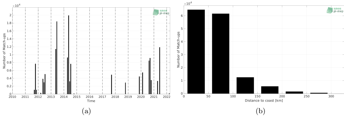
Figure 1: Number of match-ups between TSG (CSIC-UTM) and SMAP SSS L4 OI v2 - Monthly (IPRC) SSS as a function of time (a) and as function of the distance to coast (b) over the Mediterranean Sea Pi-MEP region and for the full satellite product period.
