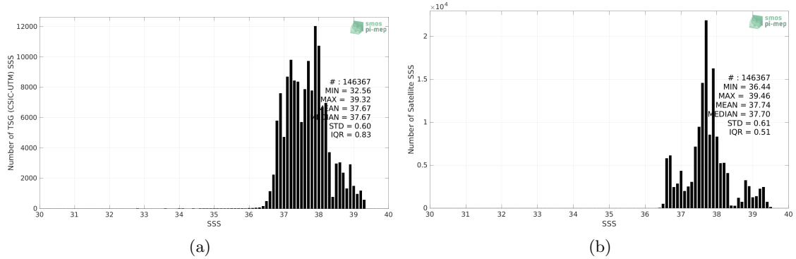
Figure 2: Histograms of SSS from TSG (CSIC-UTM) (a) and SMAP SSS L4 OI v2 - Monthly (IPRC) (b) considering all match-up pairs per bins of 0.1 over the Mediterranean Sea Pi-MEP region and for the full satellite product period.
