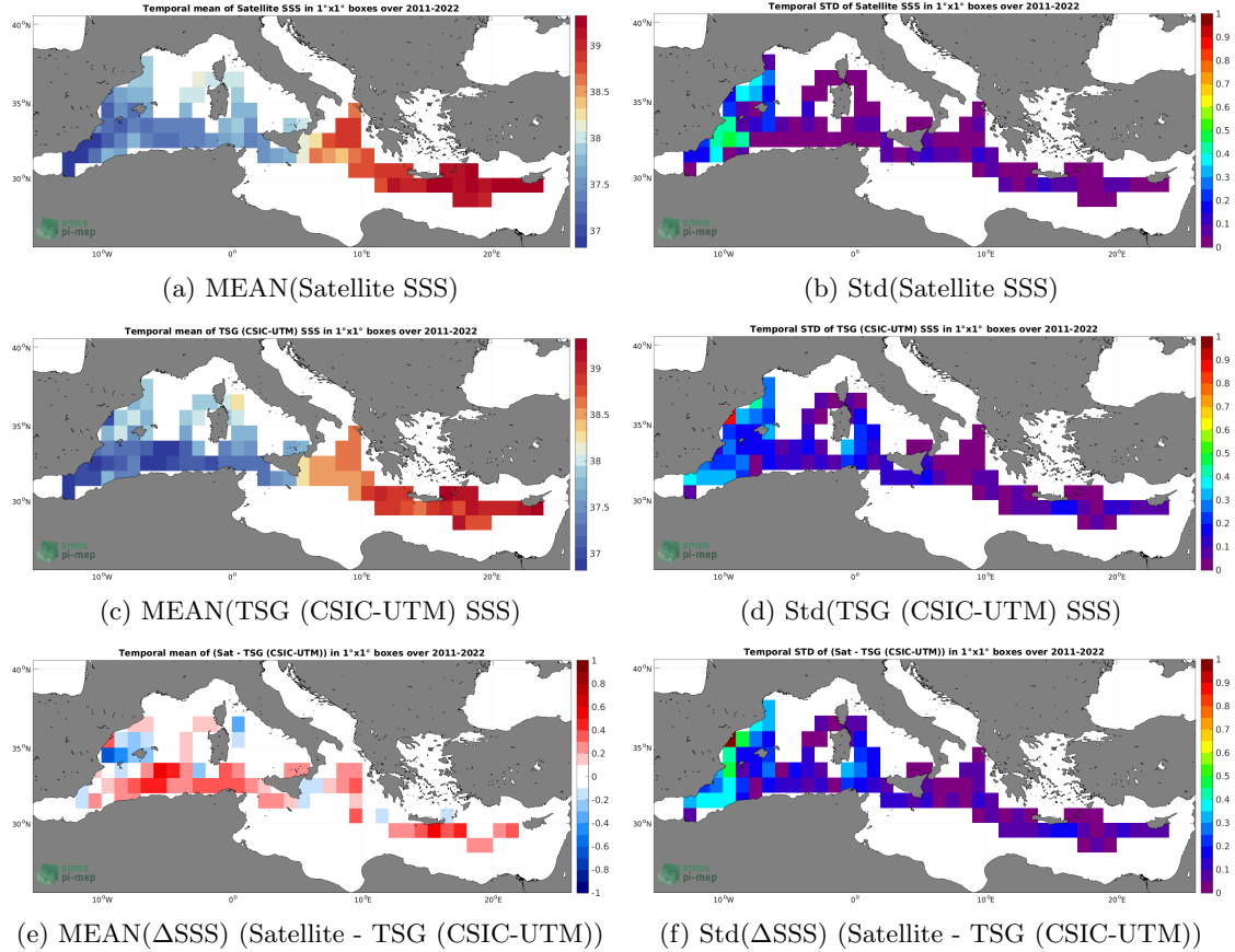
Figure 6: Temporal mean (left) and Std (right) of SSS from SMAP SSS L4 OI v2 - Monthly (IPRC) (top), TSG (CSIC-UTM) (middle), and of \Delta\text{SSS} (Satellite - TSG (CSIC-UTM)). Only match-up pairs are used to generate these maps.
