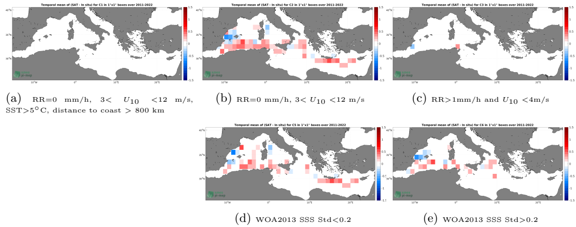
Figure 12: Temporal mean gridded over spatial boxes of size 1^\circ \times 1^\circ of \Delta SSS (SMAP SSS L4 OI v2 - Monthly (IPRC) - TSG (CSIC-UTM)) for 5 different subdatasets corresponding to:RR=0 mm/h, 3 < U_{10} < 12 m/s, SST >5^\circ\text{C} , distance to coast > 800 km (a), RR=0 mm/h, 3 < U_{10} < 12 m/s (b), RR >1 mm/h and U_{10} < 4 m/s (c), WOA2013 SSS Std <0.2 (d), WOA2013 SSS Std >0.2 (e).
