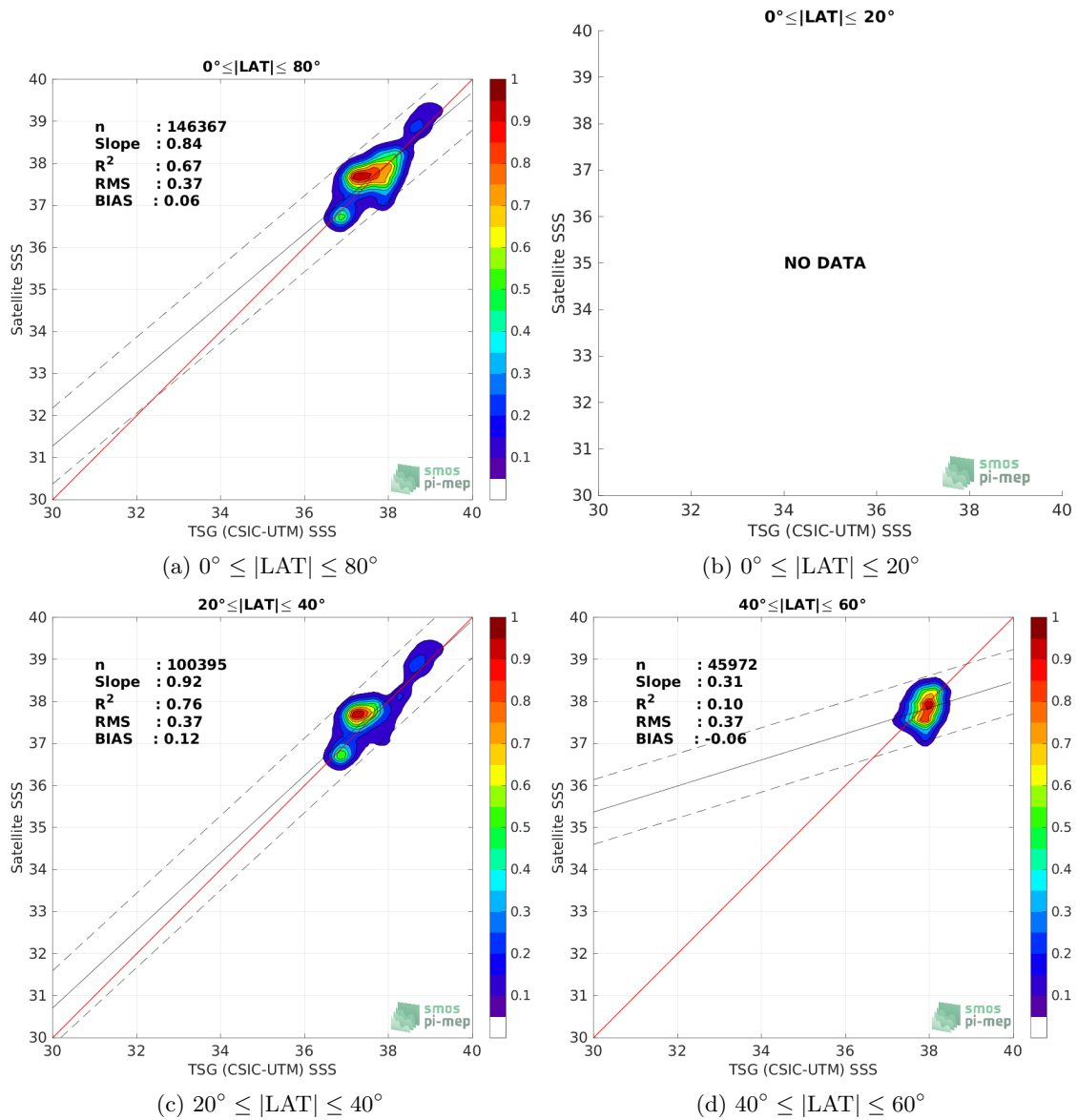
Figure 9: Contour maps of the concentration of SMAP SSS L4 OI v2 - Monthly (IPRC) SSS (y-axis) versus TSG (CSIC-UTM) SSS (x-axis) at match-up pairs for different latitude bands. For each plot, the red line shows x=y . The black thin and dashed lines indicate a linear fit through the data cloud and the \pm 95\% confidence levels, respectively. The number match-up pairs n , the slope and R^2 coefficient of the linear fit, the root mean square (RMS) and the mean bias between satellite and in situ data are indicated for each latitude band in each plots.
