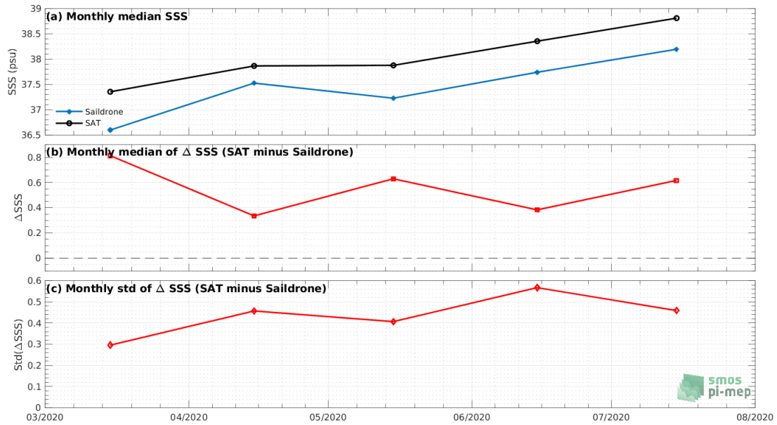
Figure 7: Time series of the monthly median SSS (top), median of \Delta SSS (Satellite - Sairdrones) and Std of \Delta SSS (Satellite - Sairdrones) over the Mediterranean Sea Pi-MEP region considering all match-ups collected by the Pi-MEP.
