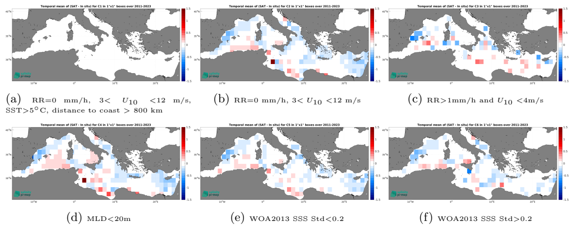
Figure 12: Temporal mean gridded over spatial boxes of size 1^\circ \times 1^\circ of \Delta SSS (SMAP SSS L4 OI v2 - Monthly (IPRC) - Argo) for 6 different subdatasets corresponding to:RR=0 mm/h, 3 < U_{10} < 12 m/s, SST >5^\circ C, distance to coast > 800 km (a), RR=0 mm/h, 3 < U_{10} < 12 m/s (b), RR >1 mm/h and U_{10} < 4 m/s (c),MLD <20 m (d),WOA2013 SSS Std <0.2 (e),WOA2013 SSS Std >0.2 (f).
