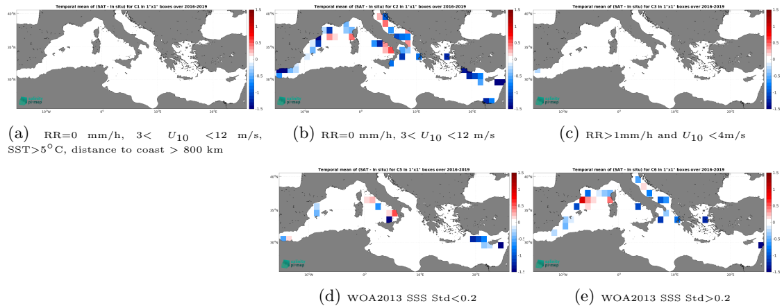
Figure 14: Temporal mean gridded over spatial boxes of size 1^\circ \times 1^\circ of \Delta\text{SSS} (SMAP SSS L3 v6 - 8-Day running (RSS) - TSG (GOSUD-Sailing-ship)) for 5 different subdatasets corresponding to:RR=0 mm/h, 3 < U_{10} < 12 m/s, SST >5^\circ\text{C} , distance to coast > 800 km (a), RR=0 mm/h, 3 < U_{10} < 12 m/s (b), RR >1 mm/h and U_{10} < 4 m/s (c), WOA2013 SSS Std <0.2 (d), WOA2013 SSS Std >0.2 (e).
