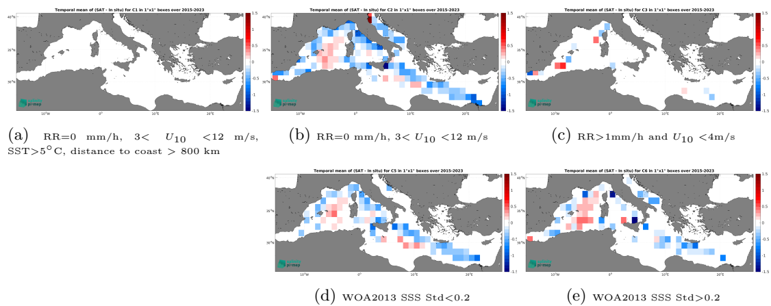
Figure 14: Temporal mean gridded over spatial boxes of size 1^\circ \times 1^\circ of \Delta SSS (SMAP SSS L3 v6 - Monthly (RSS) - TSG (LEGOS-DM)) for 5 different subdatasets corresponding to:RR=0 mm/h, 3 < U_{10} < 12 m/s, SST >5^\circ\text{C} , distance to coast > 800 km (a), RR=0 mm/h, 3 < U_{10} < 12 m/s (b), RR >1 mm/h and U_{10} < 4 m/s (c), WOA2013 SSS Std <0.2 (d), WOA2013 SSS Std >0.2 (e).
