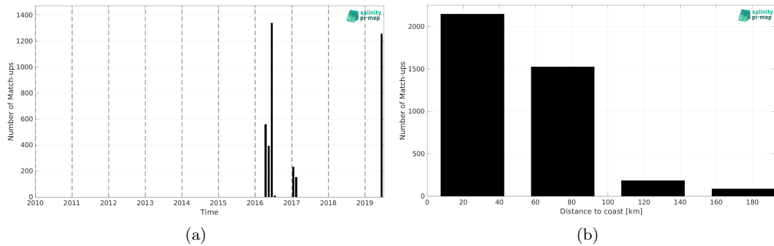
Figure 2: Number of match-ups between TSG (GOSUD-Sailing-ship) and SMAP SSS L3 v6 - Monthly (RSS) SSS as a function of time (a) and as function of the distance to coast (b) over the Mediterranean Sea Pi-MEP region and for the full satellite product period.
