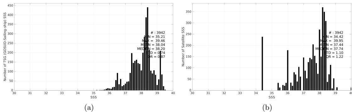
Figure 3: Histograms of SSS from TSG (GOSUD-Sailing-ship) (a) and SMAP SSS L3 v6 - Monthly (RSS) (b) considering all match-up pairs per bins of 0.1 over the Mediterranean Sea Pi-MEP region and for the full satellite product period.
