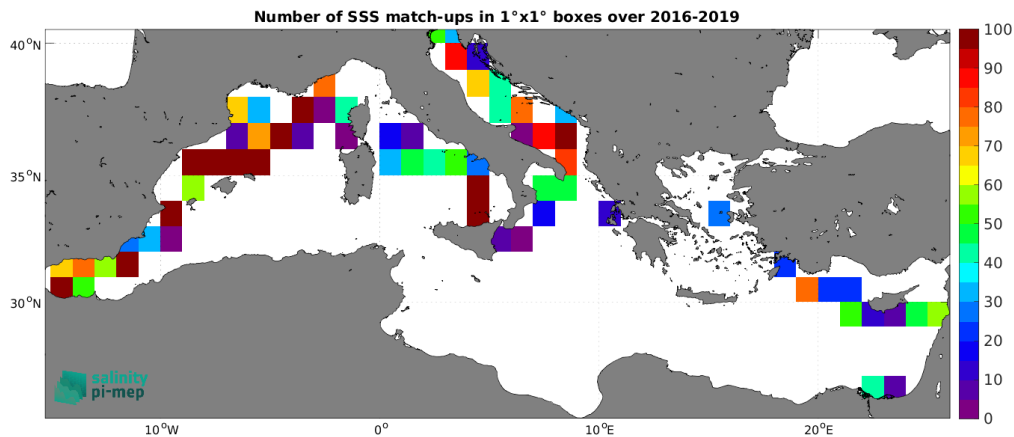
Figure 5: Number of SSS match-ups between TSG (GOSUD-Sailing-ship) SSS and the SMAP SSS L3 v6 - Monthly (RSS) SSS product for the Mediterranean Sea Pi-MEP region over 1^\circ \times 1^\circ boxes and for the full satellite product period.
