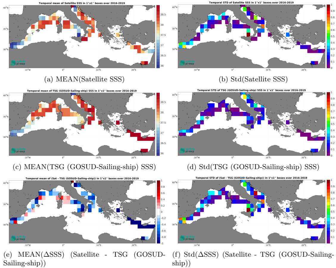
Figure 7: Temporal mean (left) and Std (right) of SSS from SMAP SSS L3 v6 - Monthly (RSS) (top), TSG (GOSUD-Sailing-ship) (middle), and of \Delta SSS (Satellite - TSG (GOSUD-Sailing-ship)). Only match-up pairs are used to generate these maps.
