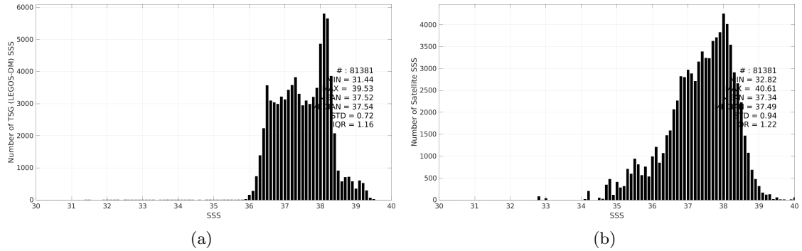
Figure 3: Histograms of SSS from TSG (LEGOS-DM) (a) and SMAP SSS L3 v5.3 - 8-Day running (RSS) (b) considering all match-up pairs per bins of 0.1 over the Mediterranean Sea Pi-MEP region and for the full satellite product period.
