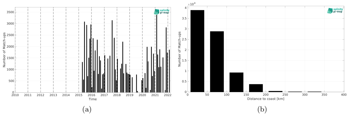
Figure 2: Number of match-ups between TSG (LEGOS-DM) and SMAP SSS L3 v5.3 - 8-Day running (RSS) SSS as a function of time (a) and as function of the distance to coast (b) over the Mediterranean Sea Pi-MEP region and for the full satellite product period.
