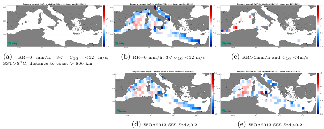
Figure 14: Temporal mean gridded over spatial boxes of size 1^\circ \times 1^\circ of \Delta\text{SSS} (SMAP SSS L3 v5.3 - 8-Day running (RSS) - TSG (LEGOS-DM)) for 5 different subdatasets corresponding to:RR=0 mm/h, 3 < U_{10} < 12 m/s, SST>5°C, distance to coast > 800 km (a), RR=0 mm/h, 3 < U_{10} < 12 m/s (b), RR>1mm/h and U_{10} < 4 m/s (c), WOA2013 SSS Std<0.2 (d), WOA2013 SSS Std>0.2 (e).
