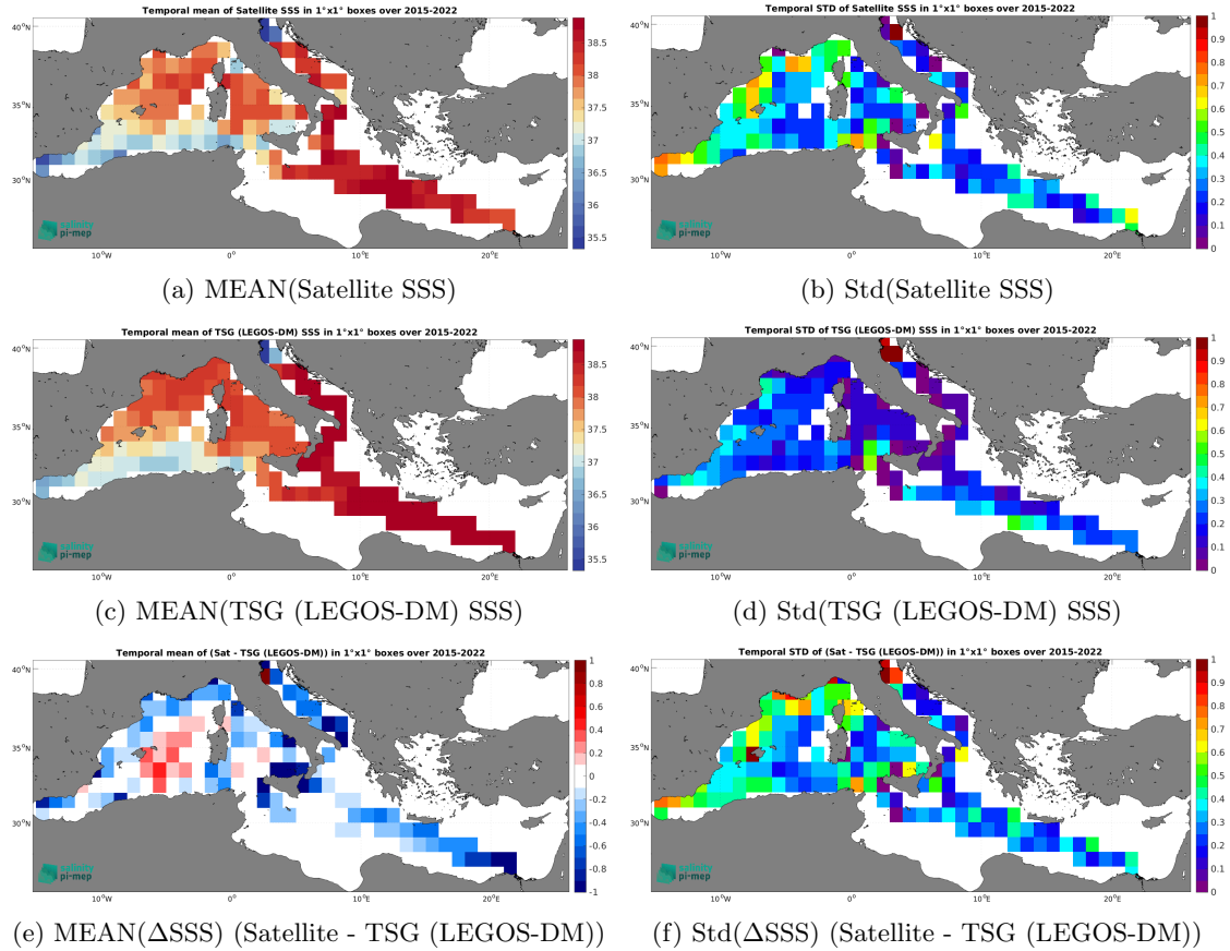
Figure 7: Temporal mean (left) and Std (right) of SSS from SMAP SSS L3 v5.3 - 8-Day running (RSS) (top), TSG (LEGOS-DM) (middle), and of \Delta\text{SSS} (Satellite - TSG (LEGOS-DM)). Only match-up pairs are used to generate these maps.
