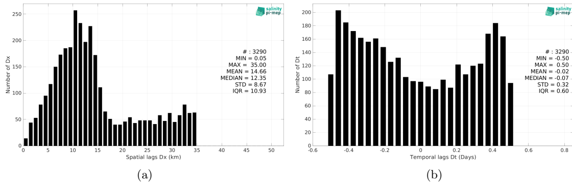
Figure 6: Histograms of the spatial (a) and temporal (b) lags between the location/time of the TSG (GOSUD-Sailing-ship) measurement and the date of the corresponding SMAP SSS L3 v5.3 - 8-Day running (RSS) SSS pixel.
