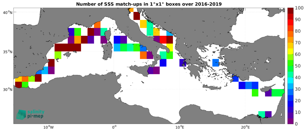
Figure 5: Number of SSS match-ups between TSG (GOSUD-Sailing-ship) SSS and the SMAP SSS L3 v5.3 - 8-Day running (RSS) SSS product for the Mediterranean Sea Pi-MEP region over 1^\circ \times 1^\circ boxes and for the full satellite product period.
