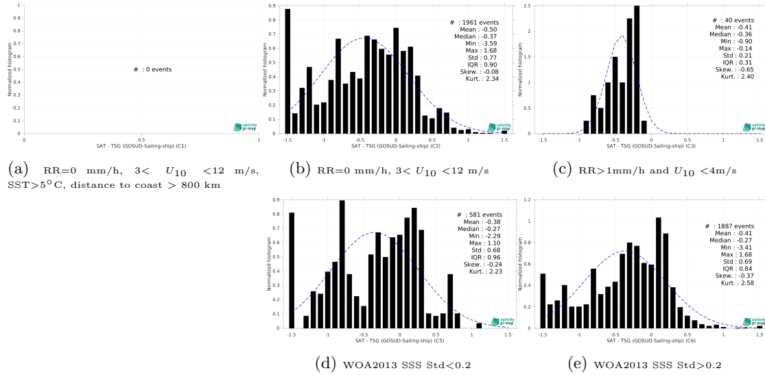
Figure 15: Normalized histogram of \Delta SSS (SMAP SSS L3 v5.3 - 8-Day running (RSS) - TSG (GOSUD-Sailing-ship)) for 5 different subdatasets corresponding to: RR=0 mm/h, 3 < U_{10} < 12 m/s, SST>5°C, distance to coast > 800 km (a), RR=0 mm/h, 3 < U_{10} < 12 m/s (b), RR>1mm/h and U_{10} < 4 m/s (c), WOA2013 SSS Std<0.2 (d), WOA2013 SSS Std>0.2 (e).
