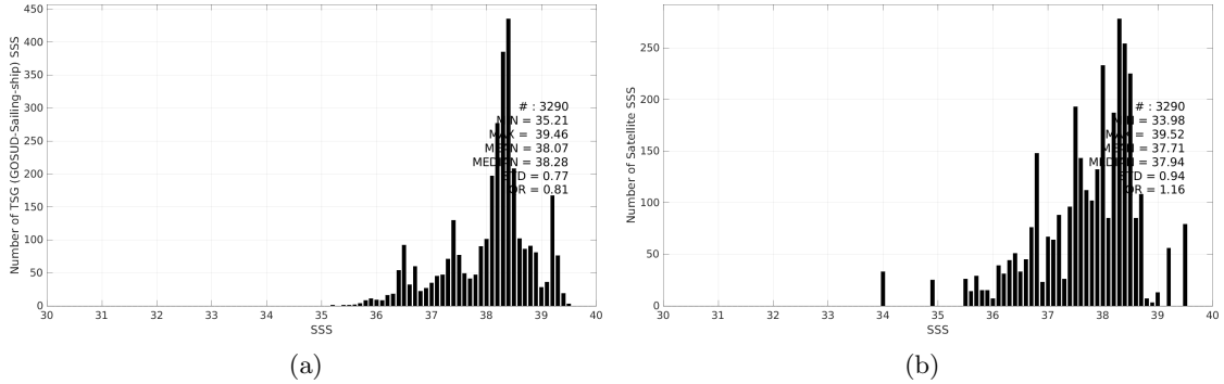
Figure 3: Histograms of SSS from TSG (GOSUD-Sailing-ship) (a) and SMAP SSS L3 v5.3 - 8-Day running (RSS) (b) considering all match-up pairs per bins of 0.1 over the Mediterranean Sea Pi-MEP region and for the full satellite product period.
