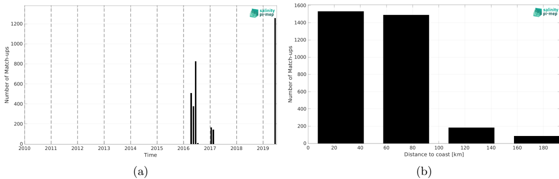
Figure 2: Number of match-ups between TSG (GOSUD-Sailing-ship) and SMAP SSS L3 v5.3 - 8-Day running (RSS) SSS as a function of time (a) and as function of the distance to coast (b) over the Mediterranean Sea Pi-MEP region and for the full satellite product period.
