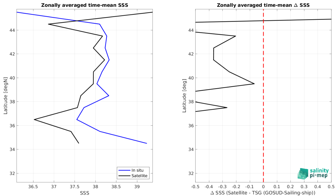
Figure 9: Left panel: Zonal mean SSS from SMAP SSS L3 v5.3 - 8-Day running (RSS) satellite product (black) and from TSG (GOSUD-Sailing-ship) (blue). Right panel: Zonal mean of \Delta SSS (Satellite - TSG (GOSUD-Sailing-ship)) for all the collected Pi-MEP match-up pairs estimated over the full satellite product period.
