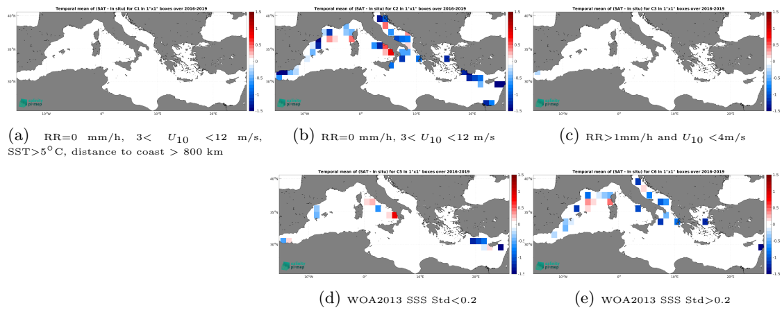
Figure 14: Temporal mean gridded over spatial boxes of size 1^\circ \times 1^\circ of \Delta\text{SSS} (SMAP SSS L3 v5.3 - 8-Day running (RSS) - TSG (GOSUD-Sailing-ship)) for 5 different subdatasets corresponding to:RR=0 mm/h, 3 < U_{10} < 12 m/s, SST >5^\circ\text{C} , distance to coast > 800 km (a), RR=0 mm/h, 3 < U_{10} < 12 m/s (b), RR >1 mm/h and U_{10} < 4 m/s (c), WOA2013 SSS Std <0.2 (d), WOA2013 SSS Std >0.2 (e).
