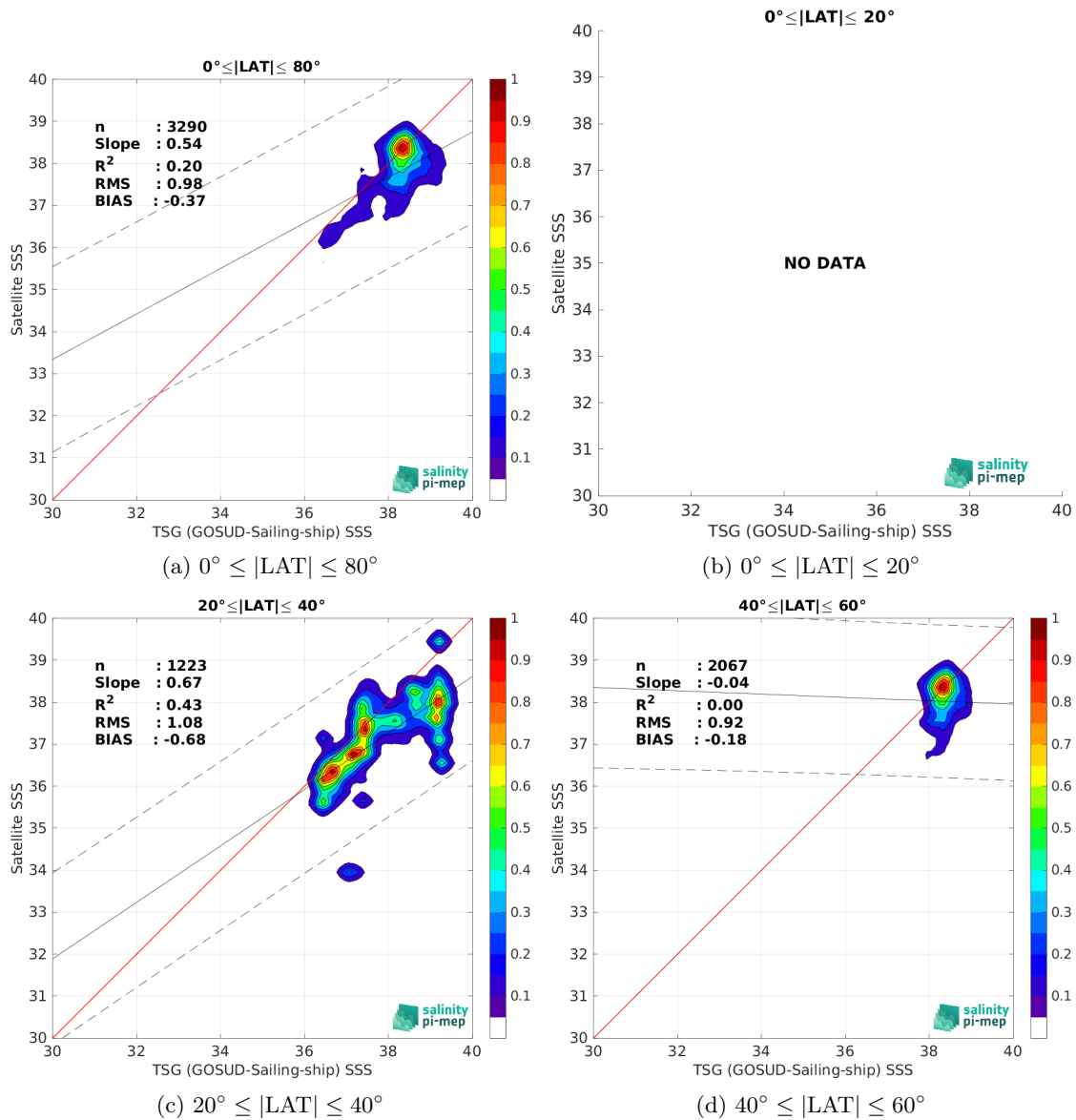
Figure 10: Contour maps of the concentration of SMAP SSS L3 v5.3 - 8-Day running (RSS) SSS (y-axis) versus TSG (GOSUD-Sailing-ship) SSS (x-axis) at match-up pairs for different latitude bands. For each plot, the red line shows x=y . The black thin and dashed lines indicate a linear fit through the data cloud and the \pm 95\% confidence levels, respectively. The number match-up pairs n , the slope and R^2 coefficient of the linear fit, the root mean square (RMS) and the mean bias between satellite and in situ data are indicated for each latitude band in each plots.
