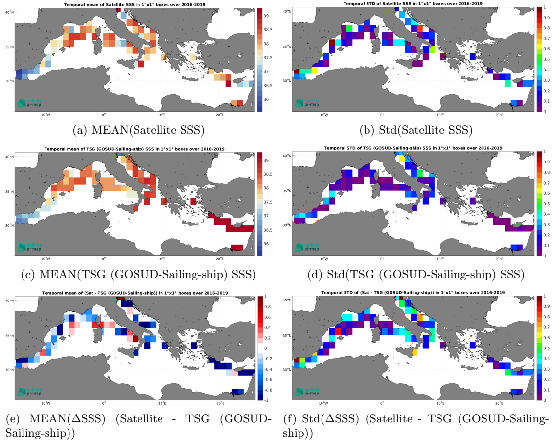
Figure 7: Temporal mean (left) and Std (right) of SSS from SMAP SSS L3 v5.3 - 8-Day running (RSS) (top), TSG (GOSUD-Sailing-ship) (middle), and of \Delta\text{SSS} (Satellite - TSG (GOSUD-Sailing-ship)). Only match-up pairs are used to generate these maps.
