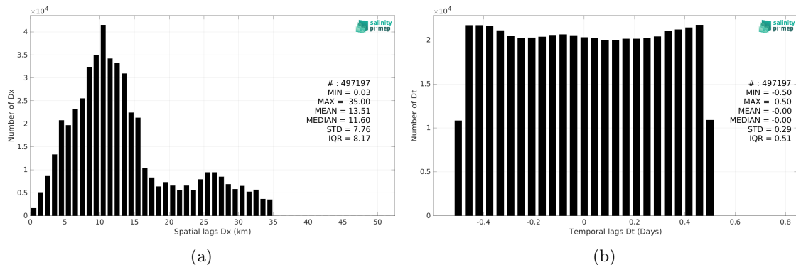
Figure 6: Histograms of the spatial (a) and temporal (b) lags between the location/time of the TSG (GOSUD-Research-vessel) measurement and the date of the corresponding SMAP SSS L3 v5.3 - 8-Day running (RSS) SSS pixel.
