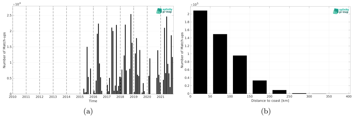
Figure 2: Number of match-ups between TSG (GOSUD-Research-vessel) and SMAP SSS L3 v5.3 - 8-Day running (RSS) SSS as a function of time (a) and as function of the distance to coast (b) over the Mediterranean Sea Pi-MEP region and for the full satellite product period.
