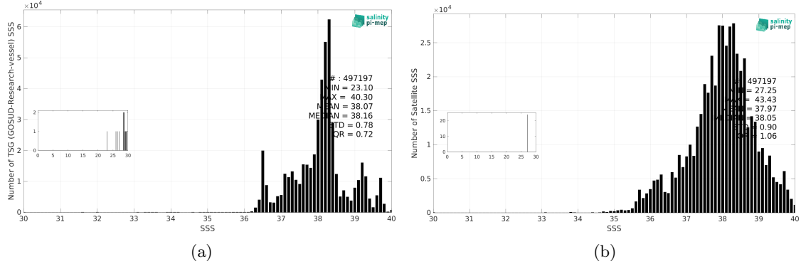
Figure 3: Histograms of SSS from TSG (GOSUD-Research-vessel) (a) and SMAP SSS L3 v5.3 - 8-Day running (RSS) (b) considering all match-up pairs per bins of 0.1 over the Mediterranean Sea Pi-MEP region and for the full satellite product period.
