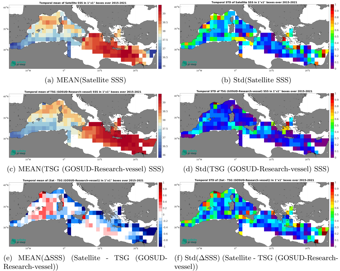
Figure 7: Temporal mean (left) and Std (right) of SSS from SMAP SSS L3 v5.3 - 8-Day running (RSS) (top), TSG (GOSUD-Research-vessel) (middle), and of \Delta\text{SSS} (Satellite - TSG (GOSUD-Research-vessel)). Only match-up pairs are used to generate these maps.
