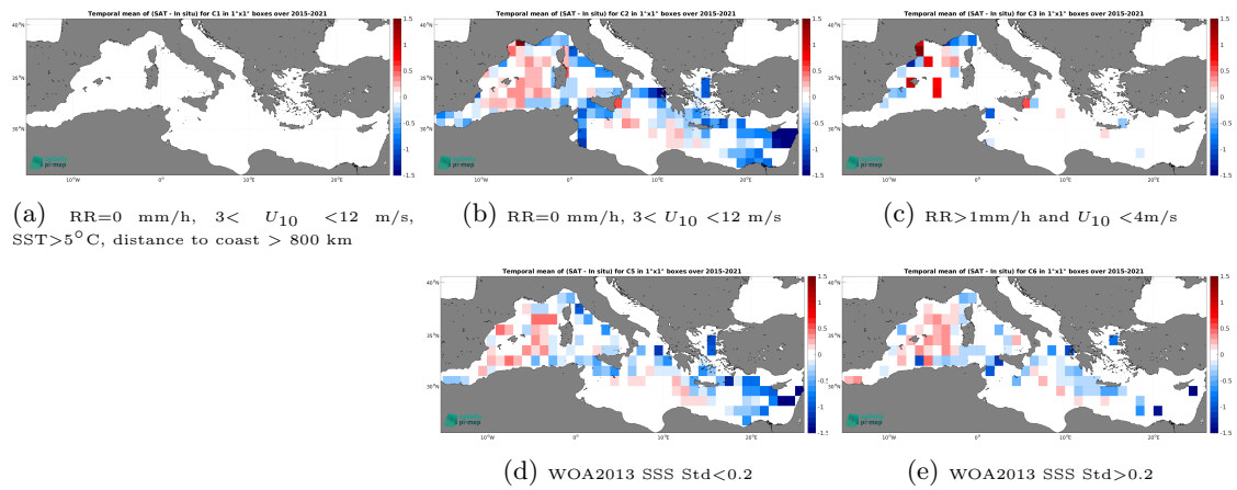
Figure 14: Temporal mean gridded over spatial boxes of size 1^\circ \times 1^\circ of \Delta SSS (SMAP SSS L3 v5.3 - 8-Day running (RSS) - TSG (GOSUD-Research-vessel)) for 5 different subdatasets corresponding to:RR=0 mm/h, 3 < U_{10} < 12 m/s, SST>5°C, distance to coast > 800 km (a), RR=0 mm/h, 3 < U_{10} < 12 m/s (b), RR>1mm/h and U_{10} < 4 m/s (c), WOA2013 SSS Std<0.2 (d), WOA2013 SSS Std>0.2 (e).
