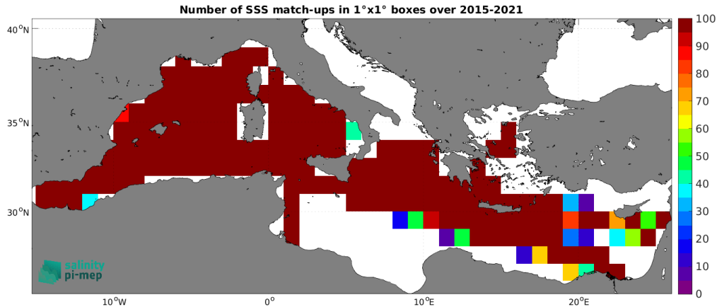
Figure 5: Number of SSS match-ups between TSG (GOSUD-Research-vessel) SSS and the SMAP SSS L3 v5.3 - 8-Day running (RSS) SSS product for the Mediterranean Sea Pi-MEP region over 1^\circ \times 1^\circ boxes and for the full satellite product period.
