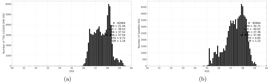
Figure 3: Histograms of SSS from TSG (LEGOS-DM) (a) and SMAP SSS L3 v5.3 - Monthly (RSS) (b) considering all match-up pairs per bins of 0.1 over the Mediterranean Sea Pi-MEP region and for the full satellite product period.
