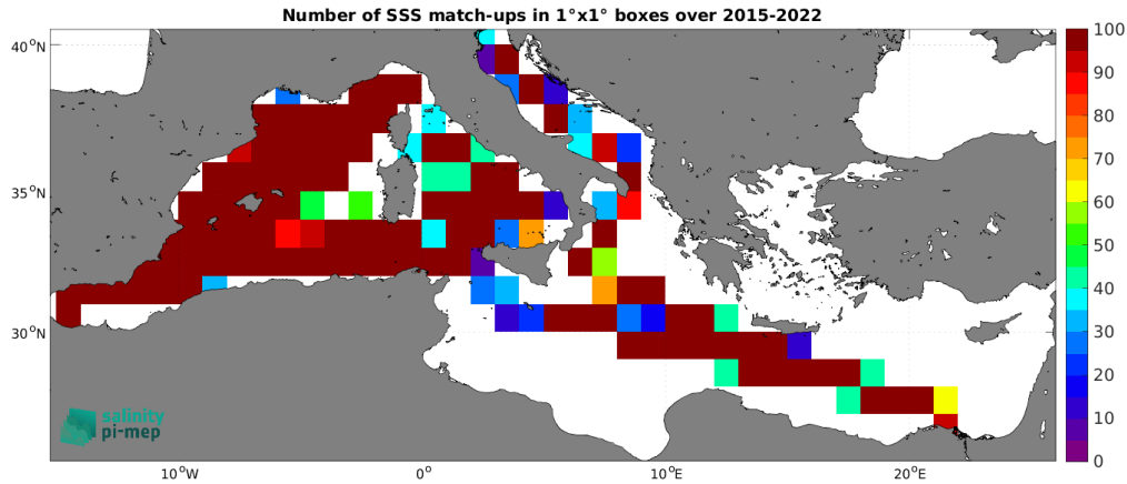
Figure 5: Number of SSS match-ups between TSG (LEGOS-DM) SSS and the SMAP SSS L3 v5.3 - Monthly (RSS) SSS product for the Mediterranean Sea Pi-MEP region over 1^\circ \times 1^\circ boxes and for the full satellite product period.
