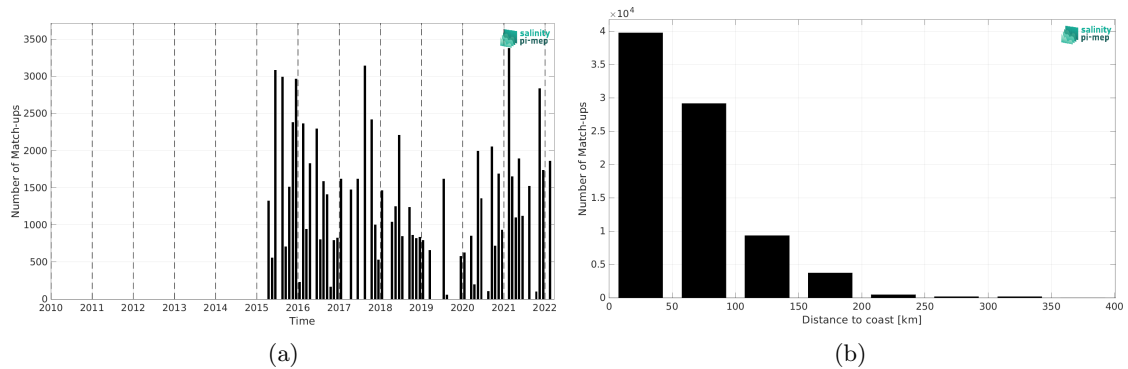
Figure 2: Number of match-ups between TSG (LEGOS-DM) and SMAP SSS L3 v5.3 - Monthly (RSS) SSS as a function of time (a) and as function of the distance to coast (b) over the Mediterranean Sea Pi-MEP region and for the full satellite product period.
