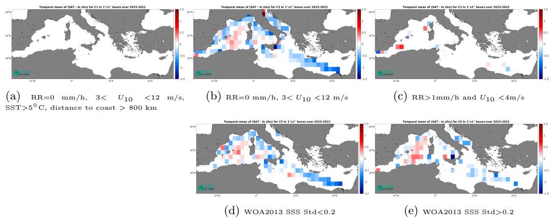
Figure 14: Temporal mean gridded over spatial boxes of size 1^\circ \times 1^\circ of \Delta SSS (SMAP SSS L3 v5.3 - Monthly (RSS) - TSG (LEGOS-DM)) for 5 different subdatasets corresponding to:RR=0 mm/h, 3 < U_{10} < 12 m/s, SST >5^\circ\text{C} , distance to coast > 800 km (a), RR=0 mm/h, 3 < U_{10} < 12 m/s (b), RR >1 mm/h and U_{10} < 4 m/s (c), WOA2013 SSS Std <0.2 (d), WOA2013 SSS Std >0.2 (e).
