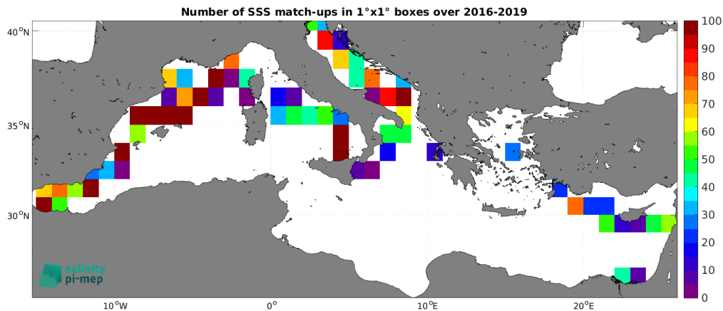
Figure 5: Number of SSS match-ups between TSG (GOSUD-Sailing-ship) SSS and the SMAP SSS L3 v5.3 - Monthly (RSS) SSS product for the Mediterranean Sea Pi-MEP region over 1^\circ \times 1^\circ boxes and for the full satellite product period.
