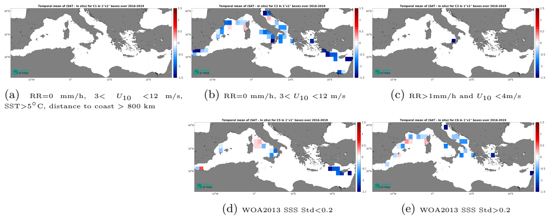
Figure 14: Temporal mean gridded over spatial boxes of size 1^\circ \times 1^\circ of \Delta SSS (SMAP SSS L3 v5.3 - Monthly (RSS) - TSG (GOSUD-Sailing-ship)) for 5 different subdatasets corresponding to:RR=0 mm/h, 3 < U_{10} < 12 m/s, SST>5°C, distance to coast > 800 km (a), RR=0 mm/h, 3 < U_{10} < 12 m/s (b), RR>1mm/h and U_{10} < 4 m/s (c), WOA2013 SSS Std<0.2 (d), WOA2013 SSS Std>0.2 (e).
