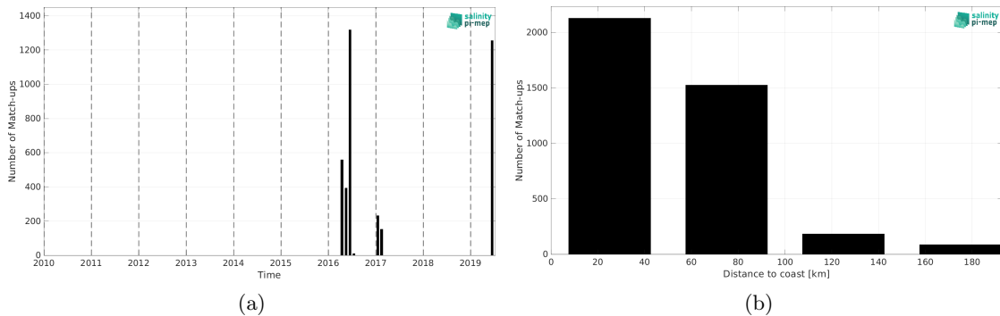
Figure 2: Number of match-ups between TSG (GOSUD-Sailing-ship) and SMAP SSS L3 v5.3 - Monthly (RSS) SSS as a function of time (a) and as function of the distance to coast (b) over the Mediterranean Sea Pi-MEP region and for the full satellite product period.
