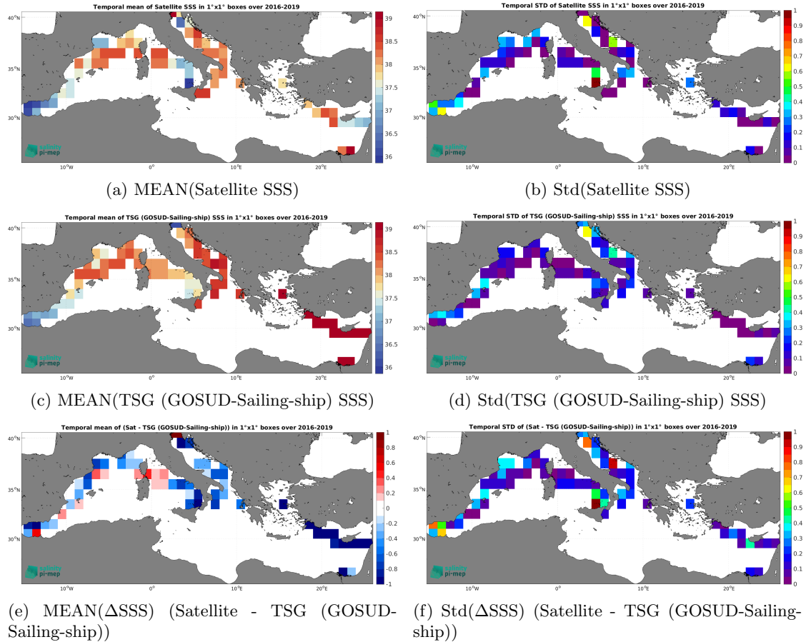
Figure 7: Temporal mean (left) and Std (right) of SSS from SMAP SSS L3 v5.3 - Monthly (RSS) (top), TSG (GOSUD-Sailing-ship) (middle), and of \Delta\text{SSS} (Satellite - TSG (GOSUD-Sailing-ship)). Only match-up pairs are used to generate these maps.
