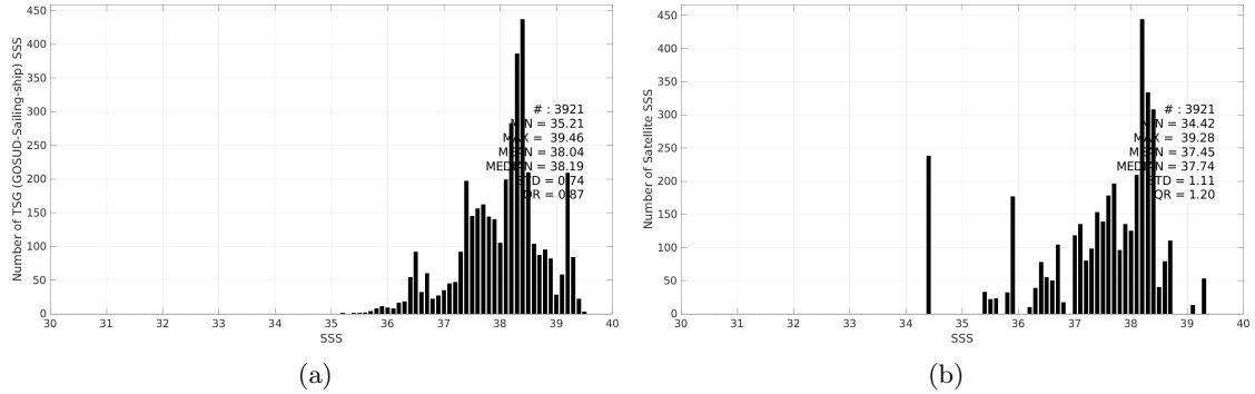
Figure 3: Histograms of SSS from TSG (GOSUD-Sailing-ship) (a) and SMAP SSS L3 v5.3 - Monthly (RSS) (b) considering all match-up pairs per bins of 0.1 over the Mediterranean Sea Pi-MEP region and for the full satellite product period.
