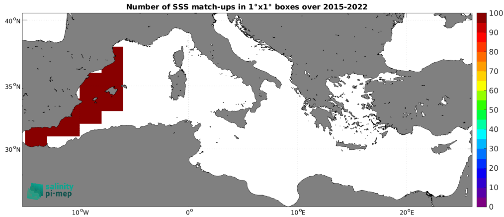
Figure 5: Number of SSS match-ups between TSG (CSIC-UTM) SSS and the SMAP SSS L3 v5.3 - Monthly (RSS) SSS product for the Mediterranean Sea Pi-MEP region over 1^\circ \times 1^\circ boxes and for the full satellite product period.
