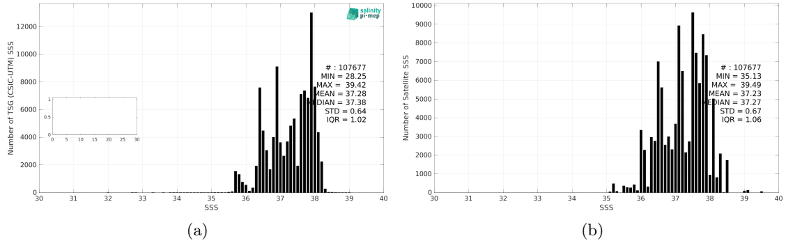
Figure 3: Histograms of SSS from TSG (CSIC-UTM) (a) and SMAP SSS L3 v5.3 - Monthly (RSS) (b) considering all match-up pairs per bins of 0.1 over the Mediterranean Sea Pi-MEP region and for the full satellite product period.
