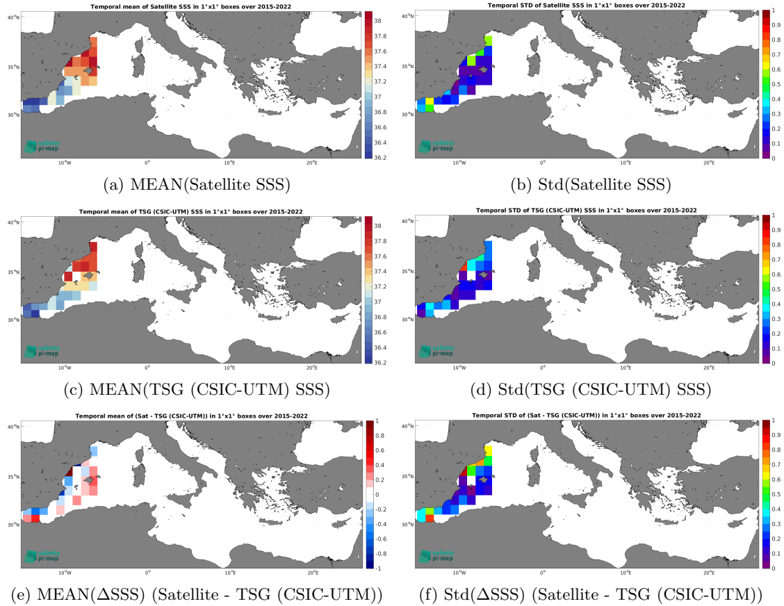
Figure 7: Temporal mean (left) and Std (right) of SSS from SMAP SSS L3 v5.3 - Monthly (RSS) (top), TSG (CSIC-UTM) (middle), and of \Delta\text{SSS} (Satellite - TSG (CSIC-UTM)). Only match-up pairs are used to generate these maps.
