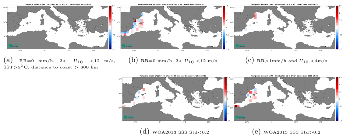
Figure 14: Temporal mean gridded over spatial boxes of size 1^\circ \times 1^\circ of \Delta\text{SSS} (SMAP SSS L3 v5.3 - Monthly (RSS) - TSG (CSIC-UTM)) for 5 different subdatasets corresponding to:RR=0 mm/h, 3 < U_{10} < 12 m/s, SST >5^\circ\text{C} , distance to coast > 800 km (a), RR=0 mm/h, 3 < U_{10} < 12 m/s (b), RR >1 mm/h and U_{10} < 4 m/s (c), WOA2013 SSS Std <0.2 (d), WOA2013 SSS Std >0.2 (e).
