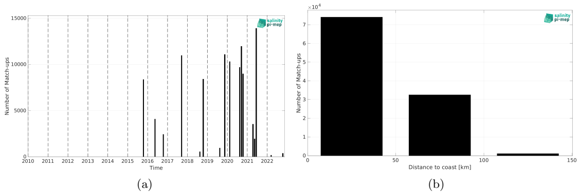
Figure 2: Number of match-ups between TSG (CSIC-UTM) and SMAP SSS L3 v5.3 - Monthly (RSS) SSS as a function of time (a) and as function of the distance to coast (b) over the Mediterranean Sea Pi-MEP region and for the full satellite product period.
