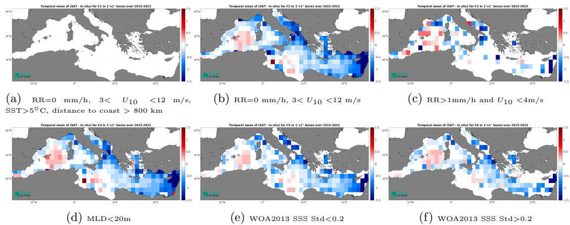
Figure 14: Temporal mean gridded over spatial boxes of size 1^\circ \times 1^\circ of \Delta SSS (SMAP SSS L3 v5.3 - Monthly (RSS) - Argo) for 6 different subdatasets corresponding to:RR=0 mm/h, 3 < U_{10} < 12 m/s, SST >5^\circ C, distance to coast > 800 km (a), RR=0 mm/h, 3 < U_{10} < 12 m/s (b), RR >1 mm/h and U_{10} < 4 m/s (c),MLD <20 m (d),WOA2013 SSS Std <0.2 (e),WOA2013 SSS Std >0.2 (f).
