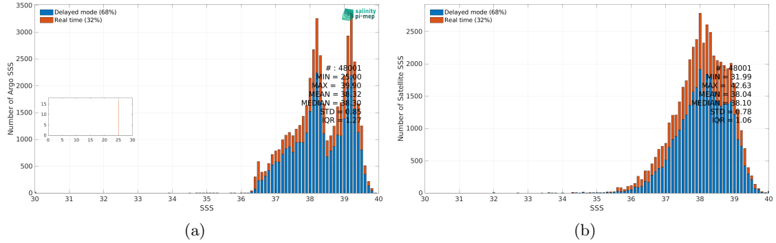
Figure 3: Histograms of SSS from Argo (a) and SMAP SSS L3 v5.3 - Monthly (RSS) (b) considering all match-up pairs per bins of 0.1 over the Mediterranean Sea Pi-MEP region and for the full satellite product period.
