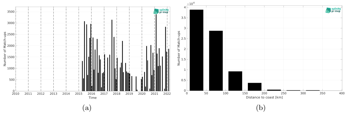
Figure 1: Number of match-ups between TSG (LEGOS-DM) and SMAP SSS L3 v5 - 8-Day running (RSS) SSS as a function of time (a) and as function of the distance to coast (b) over the Mediterranean Sea Pi-MEP region and for the full satellite product period.
