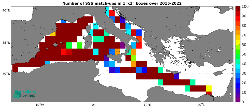
Figure 4: Number of SSS match-ups between TSG (LEGOS-DM) SSS and the SMAP SSS L3 v5 - 8-Day running (RSS) SSS product for the Mediterranean Sea Pi-MEP region over 1^\circ \times 1^\circ boxes and for the full satellite product period.
