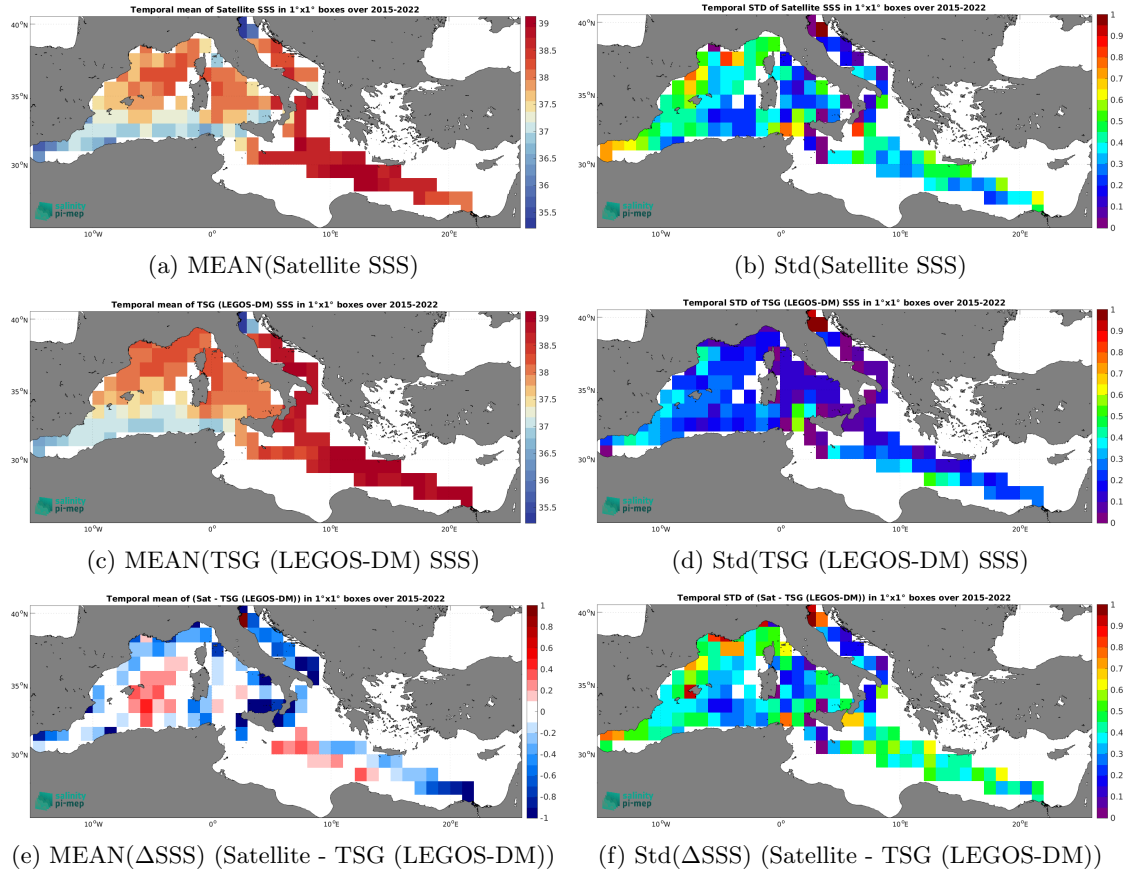
Figure 6: Temporal mean (left) and Std (right) of SSS from SMAP SSS L3 v5 - 8-Day running (RSS) (top), TSG (LEGOS-DM) (middle), and of \Delta\text{SSS} (Satellite - TSG (LEGOS-DM)). Only match-up pairs are used to generate these maps.
