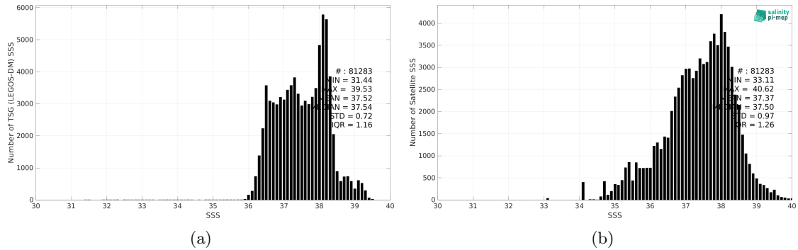
Figure 2: Histograms of SSS from TSG (LEGOS-DM) (a) and SMAP SSS L3 v5 - 8-Day running (RSS) (b) considering all match-up pairs per bins of 0.1 over the Mediterranean Sea Pi-MEP region and for the full satellite product period.
