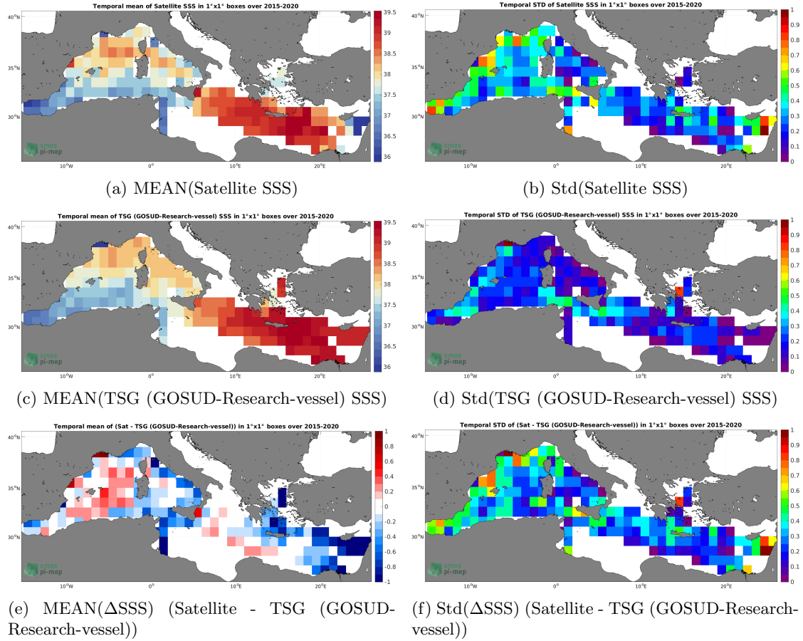
Figure 6: Temporal mean (left) and Std (right) of SSS from SMAP SSS L3 v5 - 8-Day running (RSS) (top), TSG (GOSUD-Research-vessel) (middle), and of \Delta SSS (Satellite - TSG (GOSUD-Research-vessel)). Only match-up pairs are used to generate these maps.
