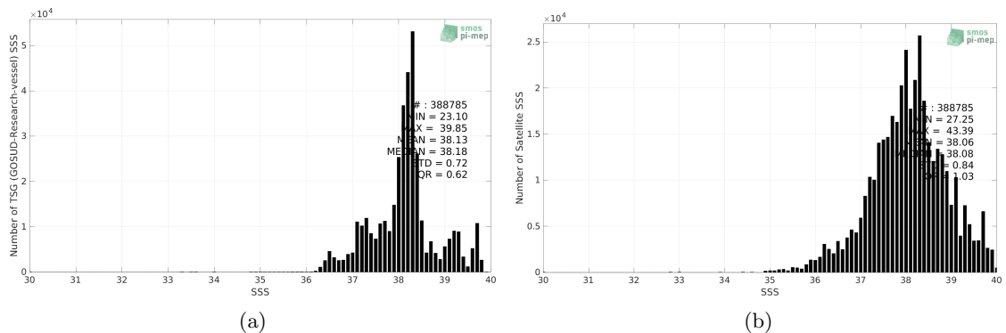
Figure 2: Histograms of SSS from TSG (GOSUD-Research-vessel) (a) and SMAP SSS L3 v5 - 8-Day running (RSS) (b) considering all match-up pairs per bins of 0.1 over the Mediterranean Sea Pi-MEP region and for the full satellite product period.
