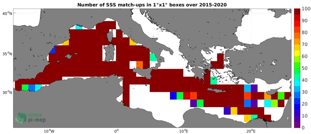
Figure 4: Number of SSS match-ups between TSG (GOSUD-Research-vessel) SSS and the SMAP SSS L3 v5 - 8-Day running (RSS) SSS product for the Mediterranean Sea Pi-MEP region over 1^\circ \times 1^\circ boxes and for the full satellite product period.
