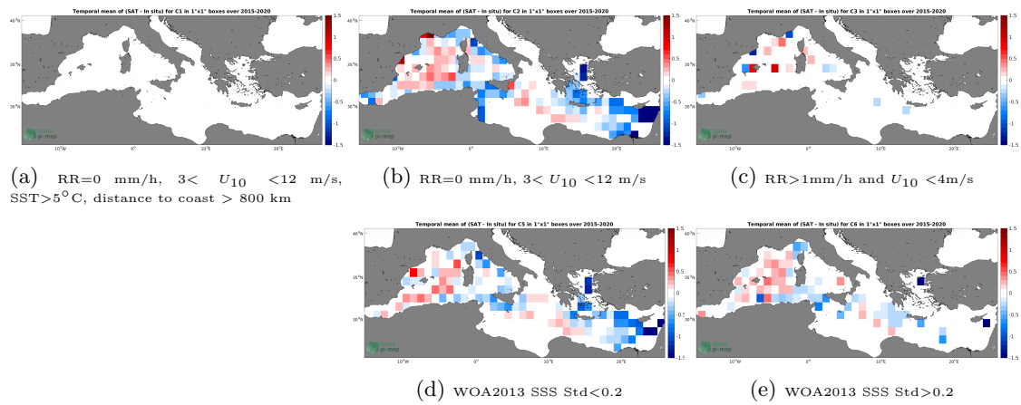
Figure 12: Temporal mean gridded over spatial boxes of size 1^\circ \times 1^\circ of \Delta\text{SSS} (SMAP SSS L3 v5 - 8-Day running (RSS) - TSG (GOSUD-Research-vessel)) for 5 different subdatasets corresponding to:RR=0 mm/h, 3 < U_{10} < 12 m/s, SST>5°C, distance to coast > 800 km (a), RR=0 mm/h, 3 < U_{10} < 12 m/s (b), RR>1mm/h and U_{10} < 4 m/s (c), WOA2013 SSS Std<0.2 (d), WOA2013 SSS Std>0.2 (e).
