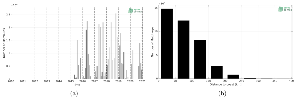
Figure 1: Number of match-ups between TSG (GOSUD-Research-vessel) and SMAP SSS L3 v5 - 8-Day running (RSS) SSS as a function of time (a) and as function of the distance to coast (b) over the Mediterranean Sea Pi-MEP region and for the full satellite product period.
