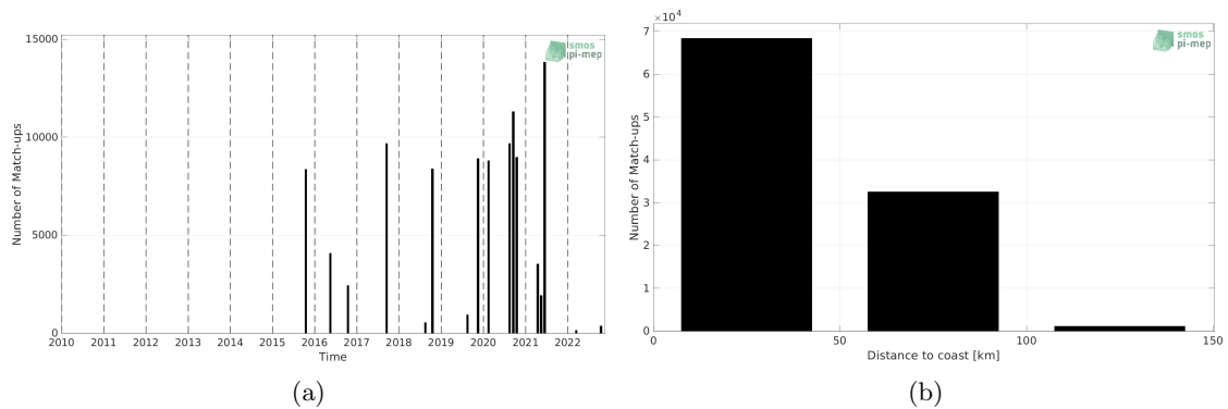
Figure 1: Number of match-ups between TSG (CSIC-UTM) and SMAP SSS L3 v5 - 8-Day running (RSS) SSS as a function of time (a) and as function of the distance to coast (b) over the Mediterranean Sea Pi-MEP region and for the full satellite product period.
