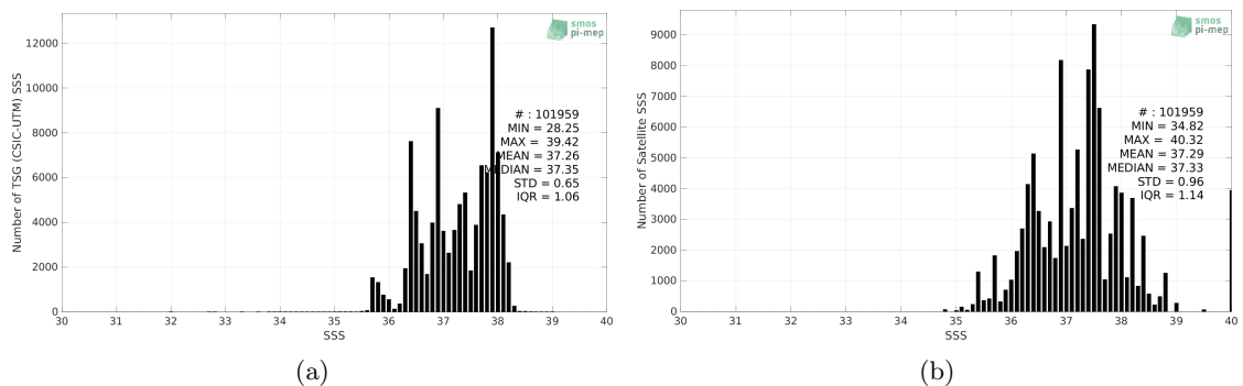
Figure 2: Histograms of SSS from TSG (CSIC-UTM) (a) and SMAP SSS L3 v5 - 8-Day running (RSS) (b) considering all match-up pairs per bins of 0.1 over the Mediterranean Sea Pi-MEP region and for the full satellite product period.
