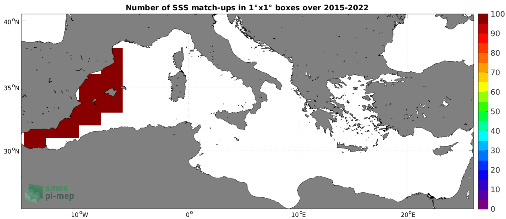
Figure 4: Number of SSS match-ups between TSG (CSIC-UTM) SSS and the SMAP SSS L3 v5 - 8-Day running (RSS) SSS product for the Mediterranean Sea Pi-MEP region over 1^\circ \times 1^\circ boxes and for the full satellite product period.
