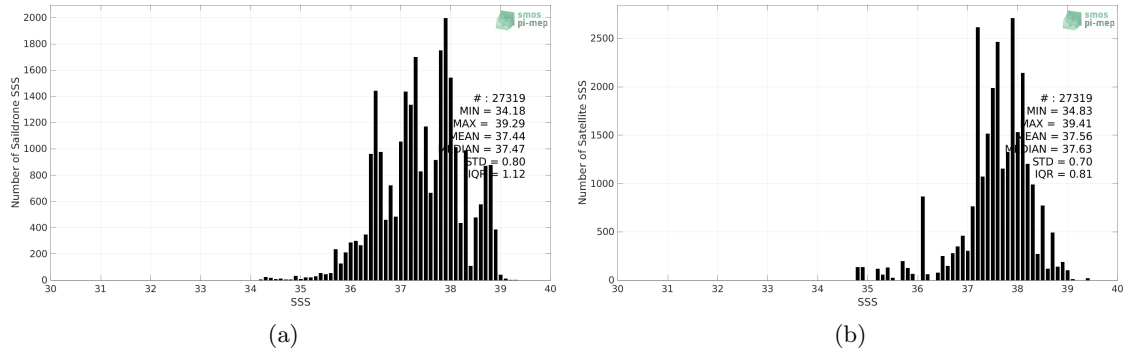
Figure 2: Histograms of SSS from Saildrone (a) and SMAP SSS L3 v5 - 8-Day running (RSS) (b) considering all match-up pairs per bins of 0.1 over the Mediterranean Sea Pi-MEP region and for the full satellite product period.
