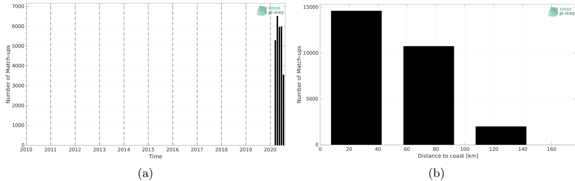
Figure 1: Number of match-ups between Saildrone and SMAP SSS L3 v5 - 8-Day running (RSS) SSS as a function of time (a) and as function of the distance to coast (b) over the Mediterranean Sea Pi-MEP region and for the full satellite product period.
