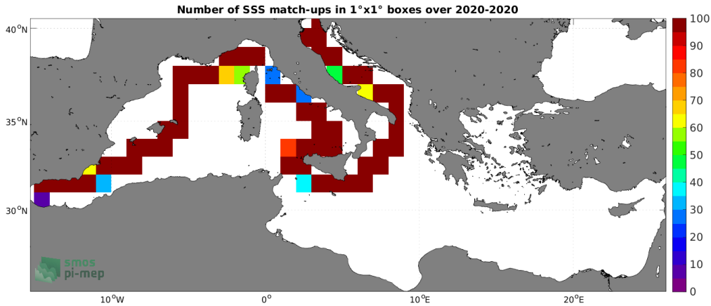
Figure 4: Number of SSS match-ups between Saildrone SSS and the SMAP SSS L3 v5 - 8-Day running (RSS) SSS product for the Mediterranean Sea Pi-MEP region over 1^\circ \times 1^\circ boxes and for the full satellite product period.
