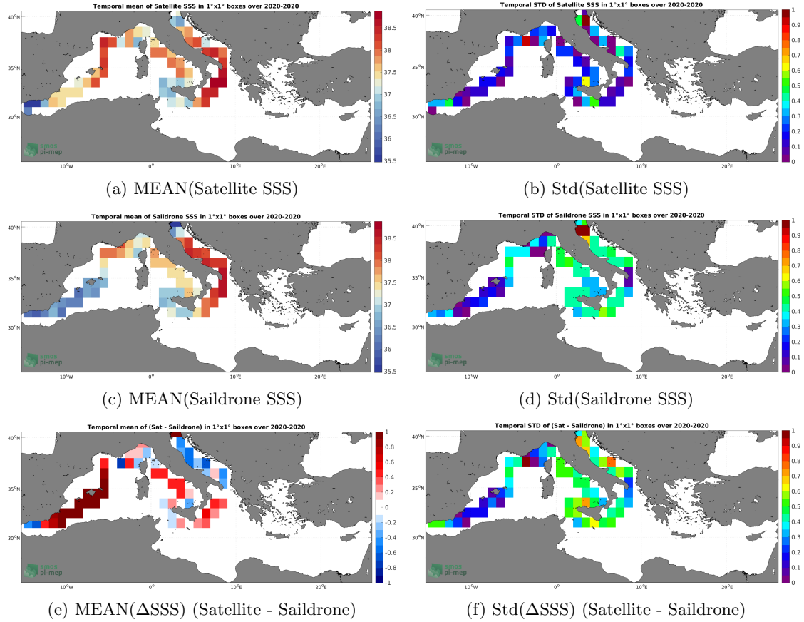
Figure 6: Temporal mean (left) and Std (right) of SSS from SMAP SSS L3 v5 - 8-Day running (RSS) (top), Saildrone (middle), and of \Delta SSS (Satellite - Saildrone). Only match-up pairs are used to generate these maps.
